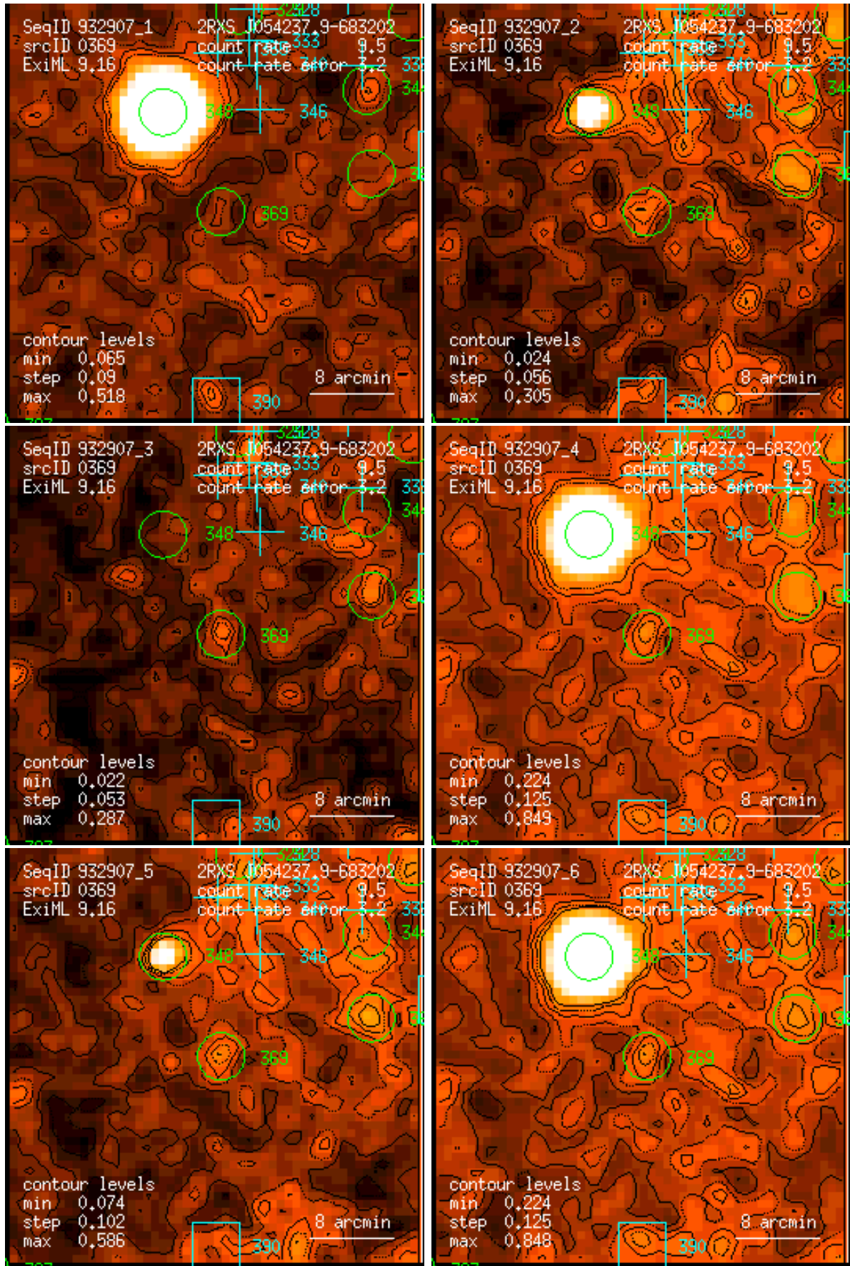
Figure 369: RASS 932907: detection 0369: band rate images, Gaussian filter: (1) PSPC channels 11 – 41, (2) 52 – 90, (3) 91 – 201, (4) 11 – 235, (5) 52 – 201, (6) 11 – 201. Broad band rates in counts/ks. Band rate contour levels in counts/ks/arcmin 2 .
