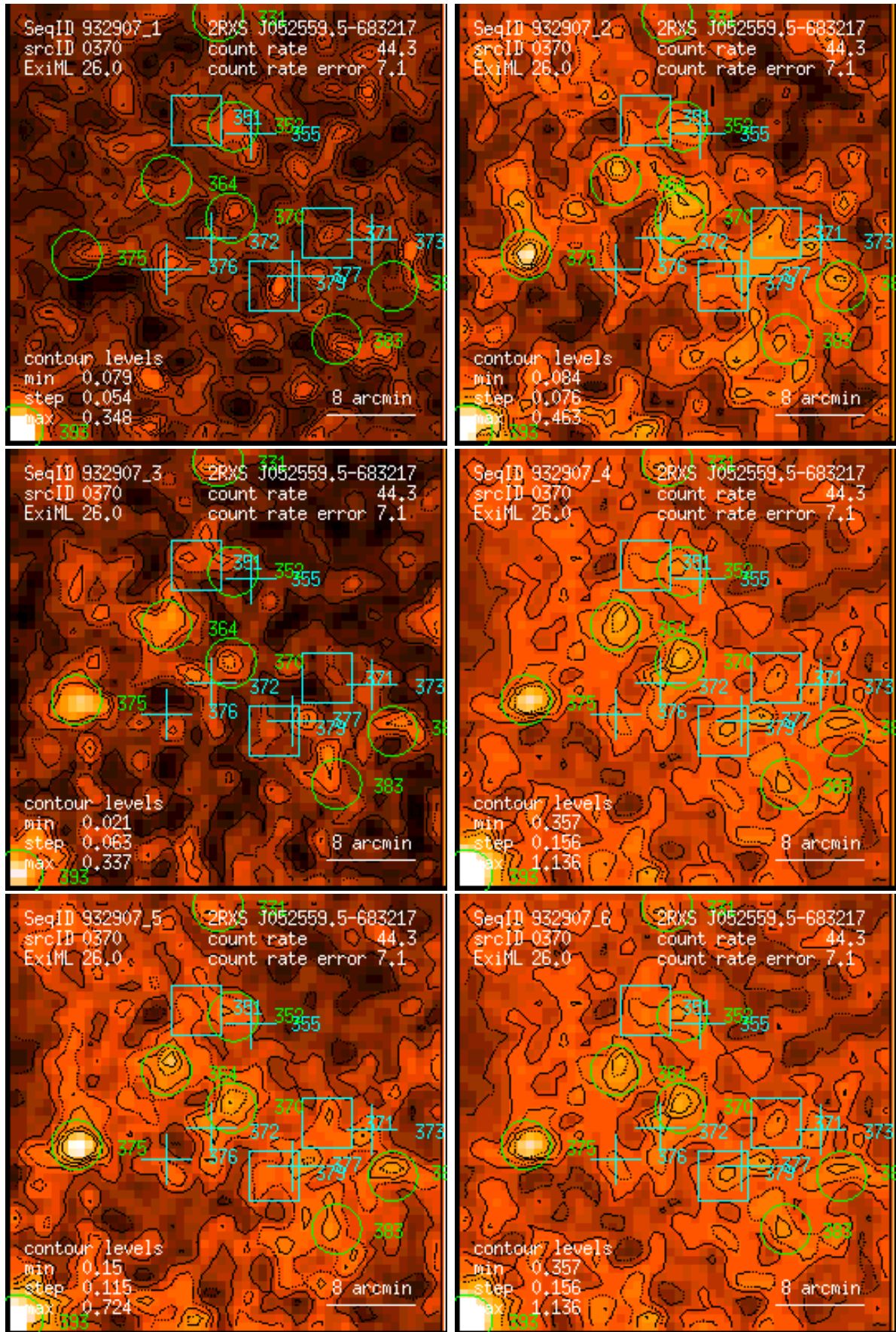
Figure 370: RASS 932907: detection 0370: band rate images, Gaussian filter: (1) PSPC channels 11 – 41, (2) 52 – 90, (3) 91 – 201, (4) 11 – 235, (5) 52 – 201, (6) 11 – 201. Broad band rates in counts/ks. Band rate contour levels in counts/ks/arcmin 2 .
