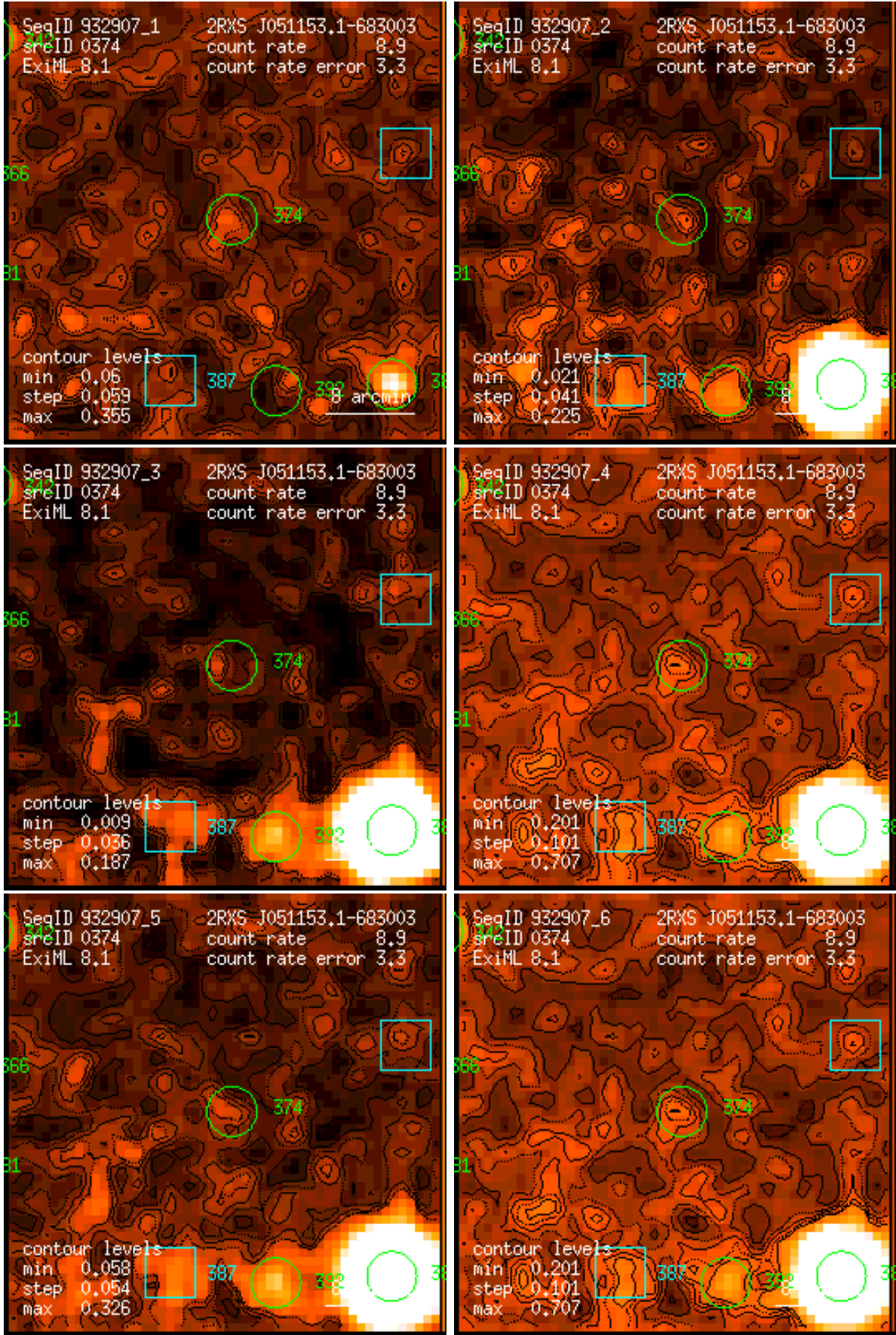
Figure 374: RASS 932907: detection 0374: band rate images, Gaussian filter: (1) PSPC channels 11 – 41, (2) 52 – 90, (3) 91 – 201, (4) 11 – 235, (5) 52 – 201, (6) 11 – 201. Broad band rates in counts/ks. Band rate contour levels in counts/ks/arcmin 2 .
