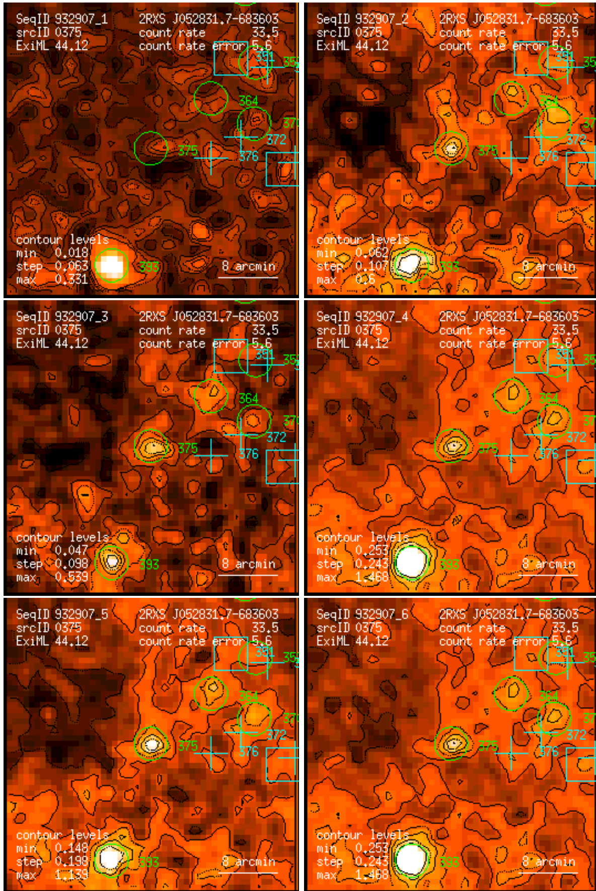
Figure 375: RASS 932907: detection 0375: band rate images, Gaussian filter: (1) PSPC channels 11 – 41, (2) 52 – 90, (3) 91 – 201, (4) 11 – 235, (5) 52 – 201, (6) 11 – 201. Broad band rates in counts/ks. Band rate contour levels in counts/ks/arcmin 2 .
