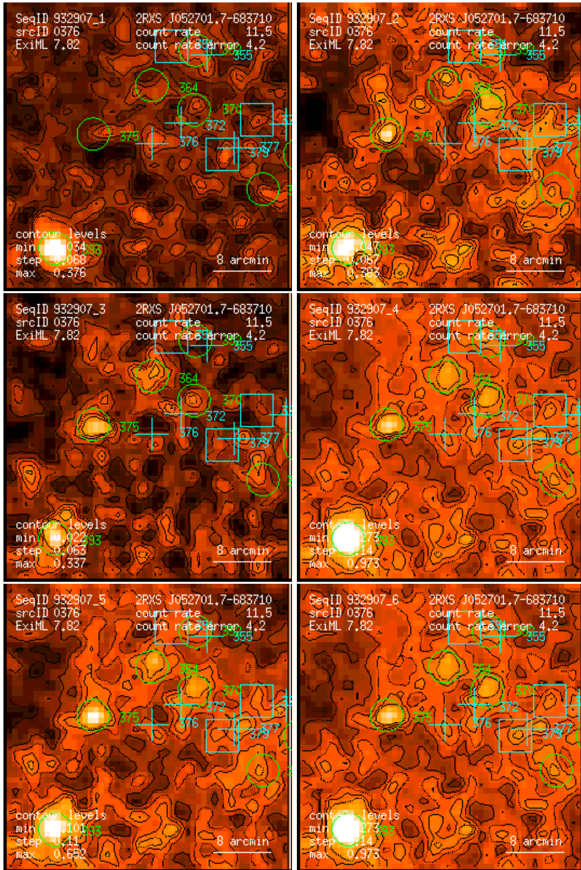
Figure 376: RASS 932907: detection 0376: band rate images, Gaussian filter: (1) PSPC channels 11 – 41, (2) 52 – 90, (3) 91 – 201, (4) 11 – 235, (5) 52 – 201, (6) 11 – 201. Broad band rates in counts/ks. Band rate contour levels in counts/ks/arcmin 2 .
