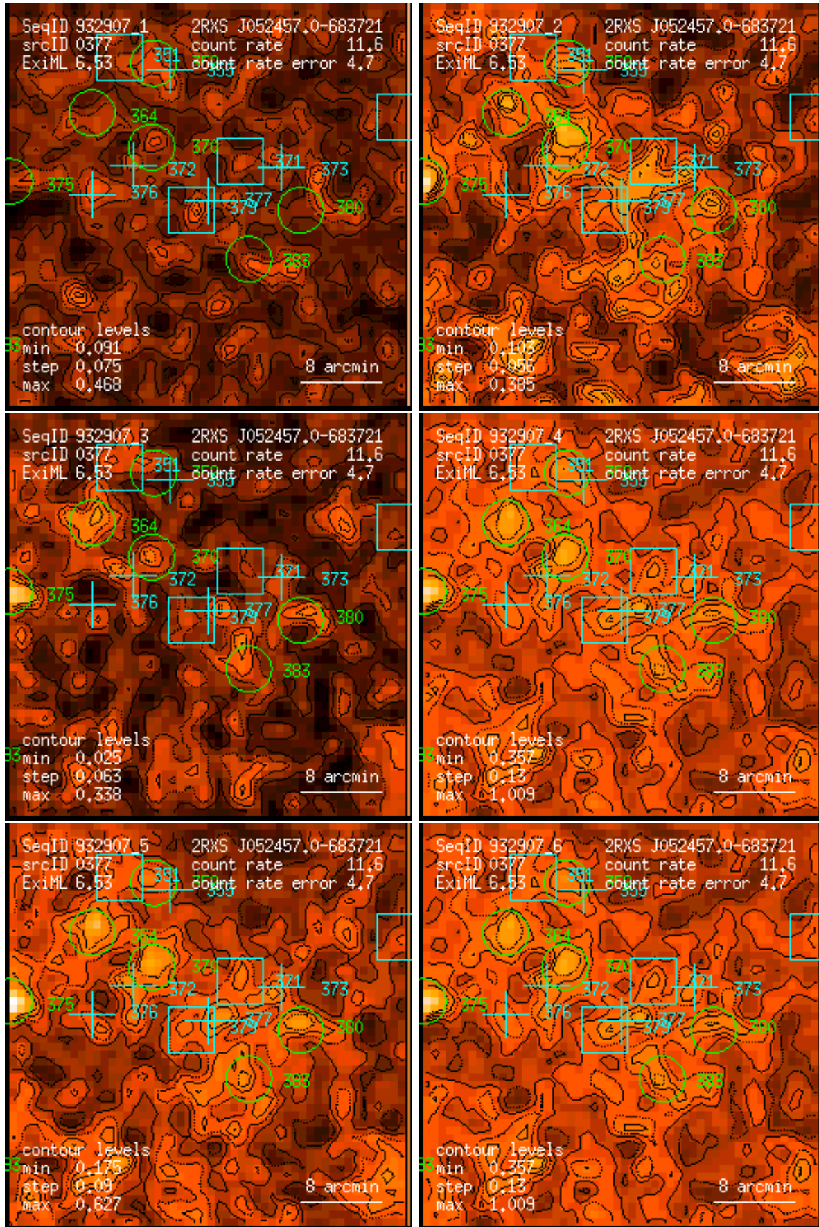
Figure 377: RASS 932907: detection 0377: band rate images, Gaussian filter: (1) PSPC channels 11 – 41, (2) 52 – 90, (3) 91 – 201, (4) 11 – 235, (5) 52 – 201, (6) 11 – 201. Broad band rates in counts/ks. Band rate contour levels in counts/ks/arcmin 2 .
