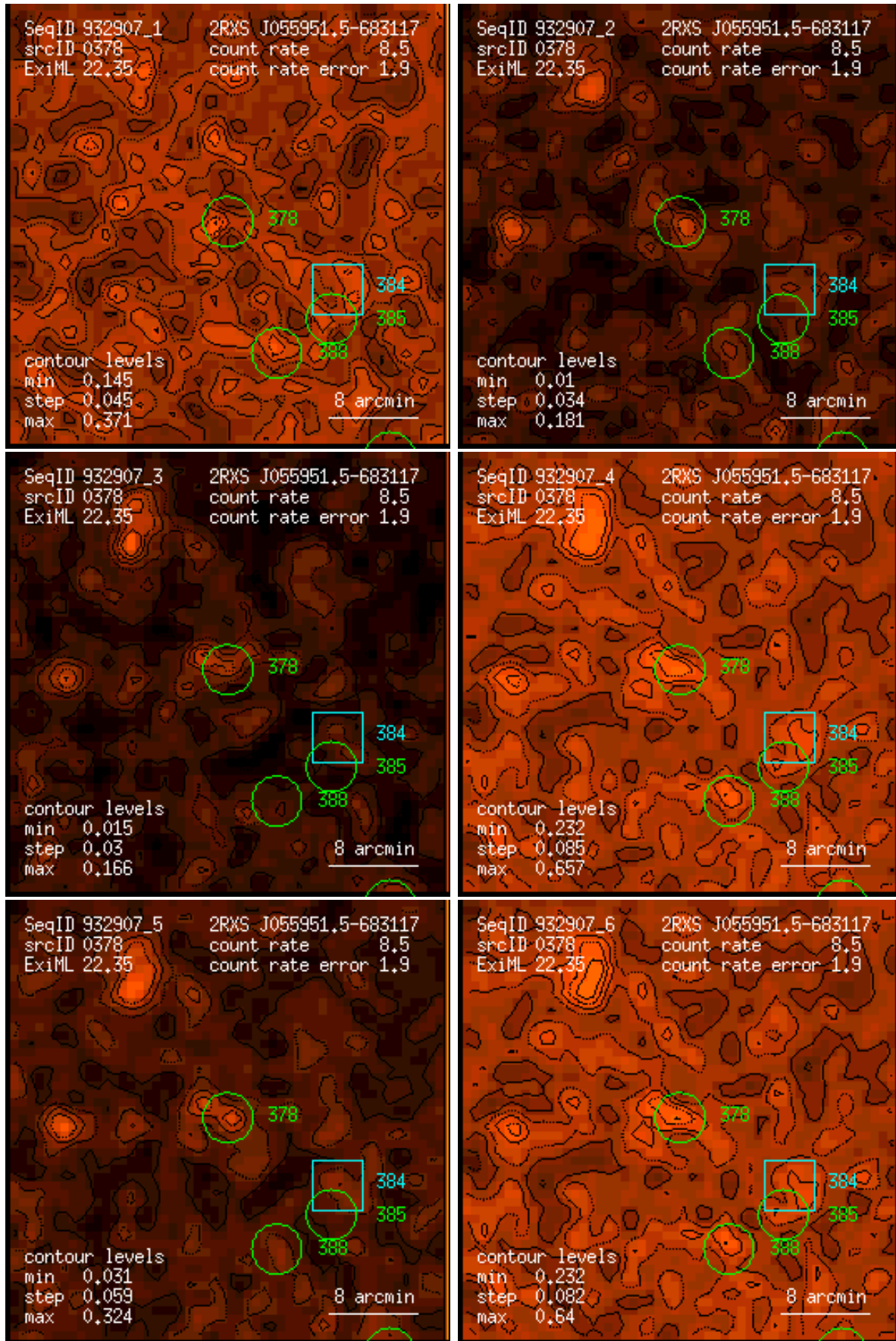
Figure 378: RASS 932907: detection 0378: band rate images, Gaussian filter: (1) PSPC channels 11 – 41, (2) 52 – 90, (3) 91 – 201, (4) 11 – 235, (5) 52 – 201, (6) 11 – 201. Broad band rates in counts/ks. Band rate contour levels in counts/ks/arcmin 2 .
