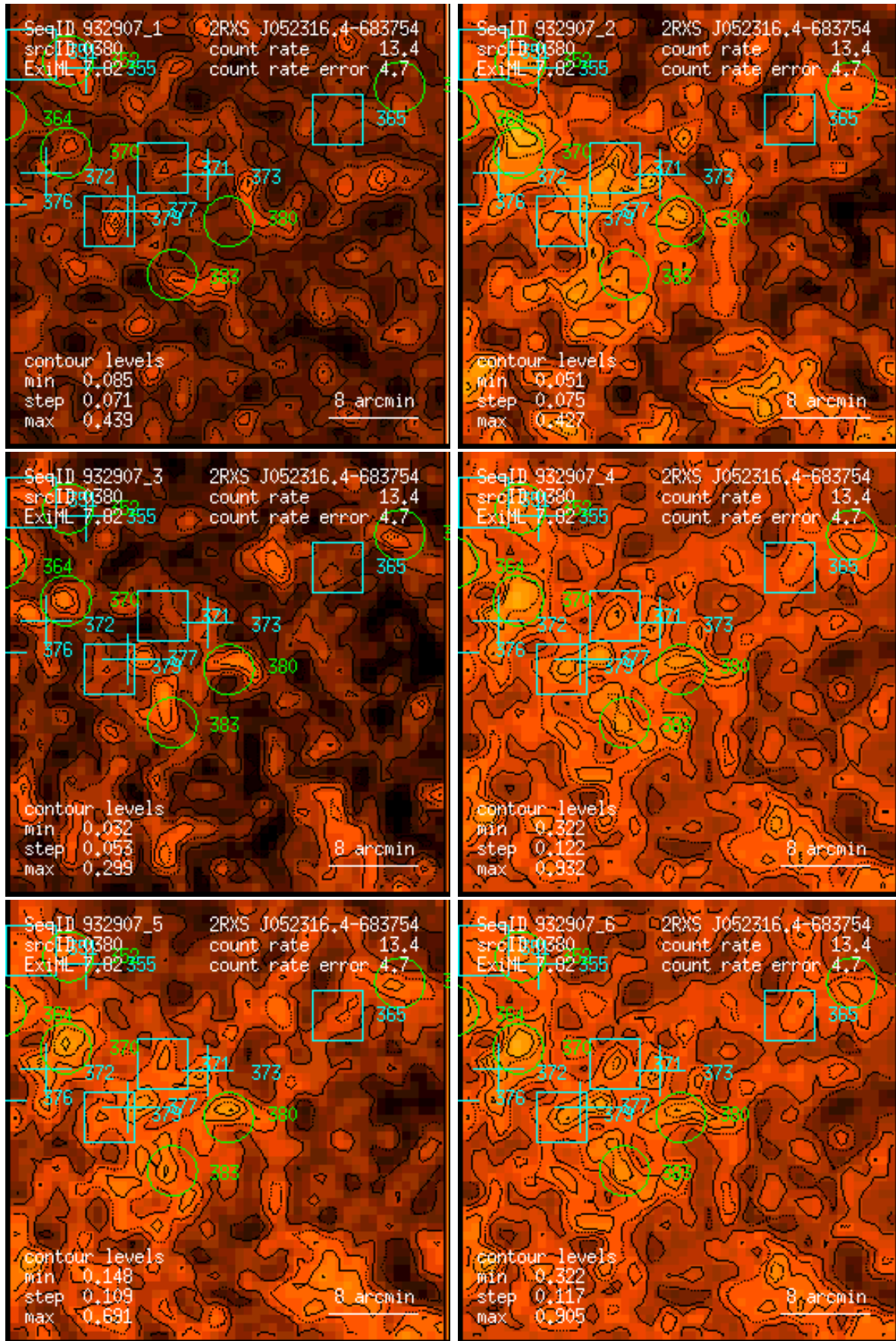
Figure 380: RASS 932907: detection 0380: band rate images, Gaussian filter: (1) PSPC channels 11 – 41, (2) 52 – 90, (3) 91 – 201, (4) 11 – 235, (5) 52 – 201, (6) 11 – 201. Broad band rates in counts/ks. Band rate contour levels in counts/ks/arcmin 2 .
