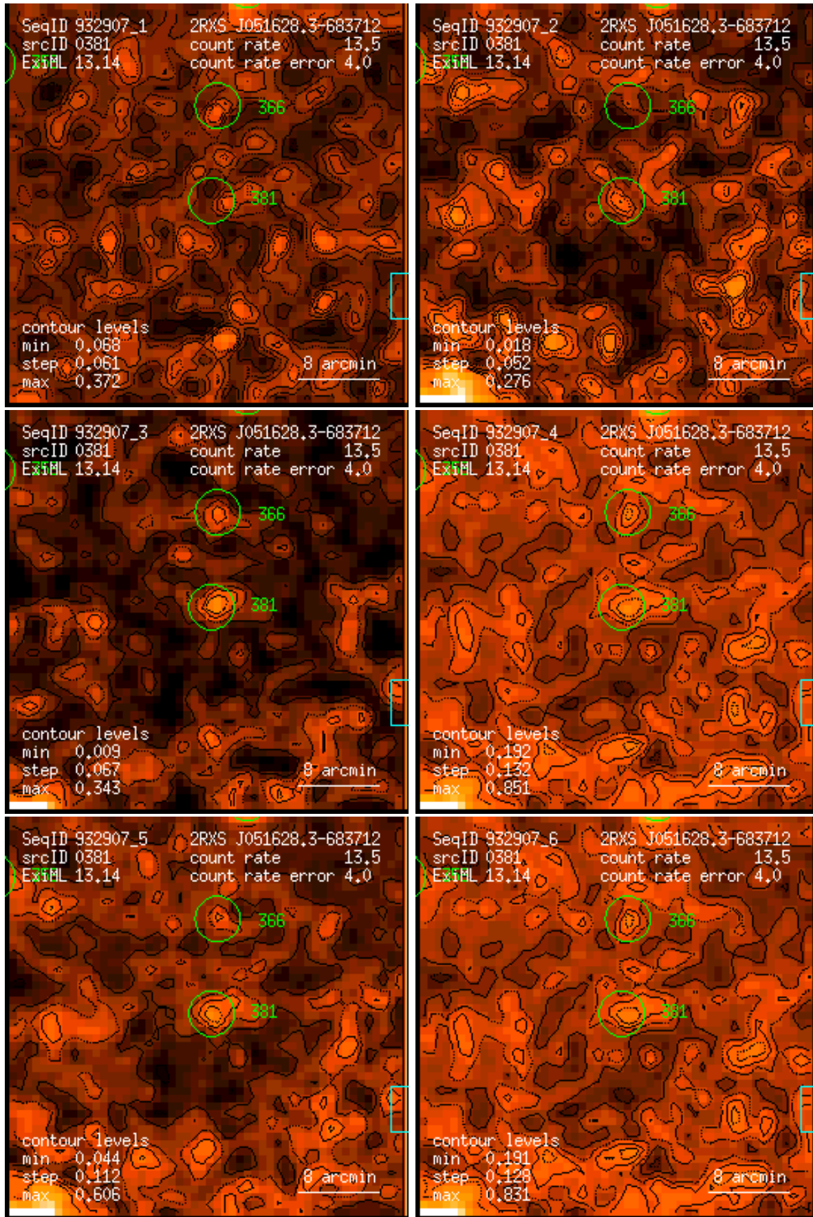
Figure 381: RASS 932907: detection 0381: band rate images, Gaussian filter: (1) PSPC channels 11 – 41, (2) 52 – 90, (3) 91 – 201, (4) 11 – 235, (5) 52 – 201, (6) 11 – 201. Broad band rates in counts/ks. Band rate contour levels in counts/ks/arcmin 2 .
