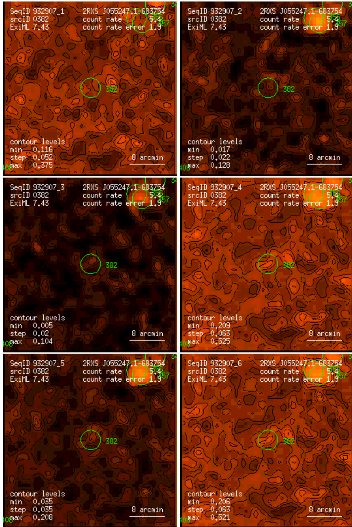
Figure 382: RASS 932907: detection 0382: band rate images, Gaussian filter: (1) PSPC channels 11 – 41, (2) 52 – 90, (3) 91 – 201, (4) 11 – 235, (5) 52 – 201, (6) 11 – 201. Broad band rates in counts/ks. Band rate contour levels in counts/ks/arcmin 2 .
