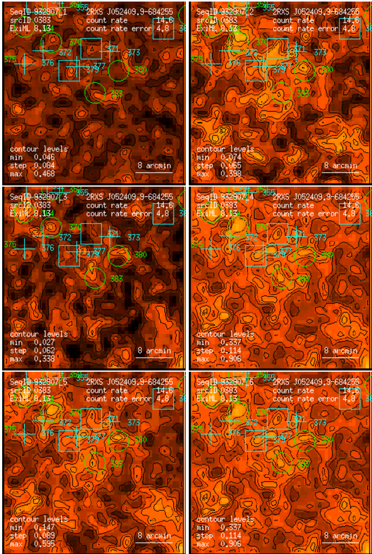
Figure 383: RASS 932907: detection 0383: band rate images, Gaussian filter: (1) PSPC channels 11 – 41, (2) 52 – 90, (3) 91 – 201, (4) 11 – 235, (5) 52 – 201, (6) 11 – 201. Broad band rates in counts/ks. Band rate contour levels in counts/ks/arcmin 2 .
