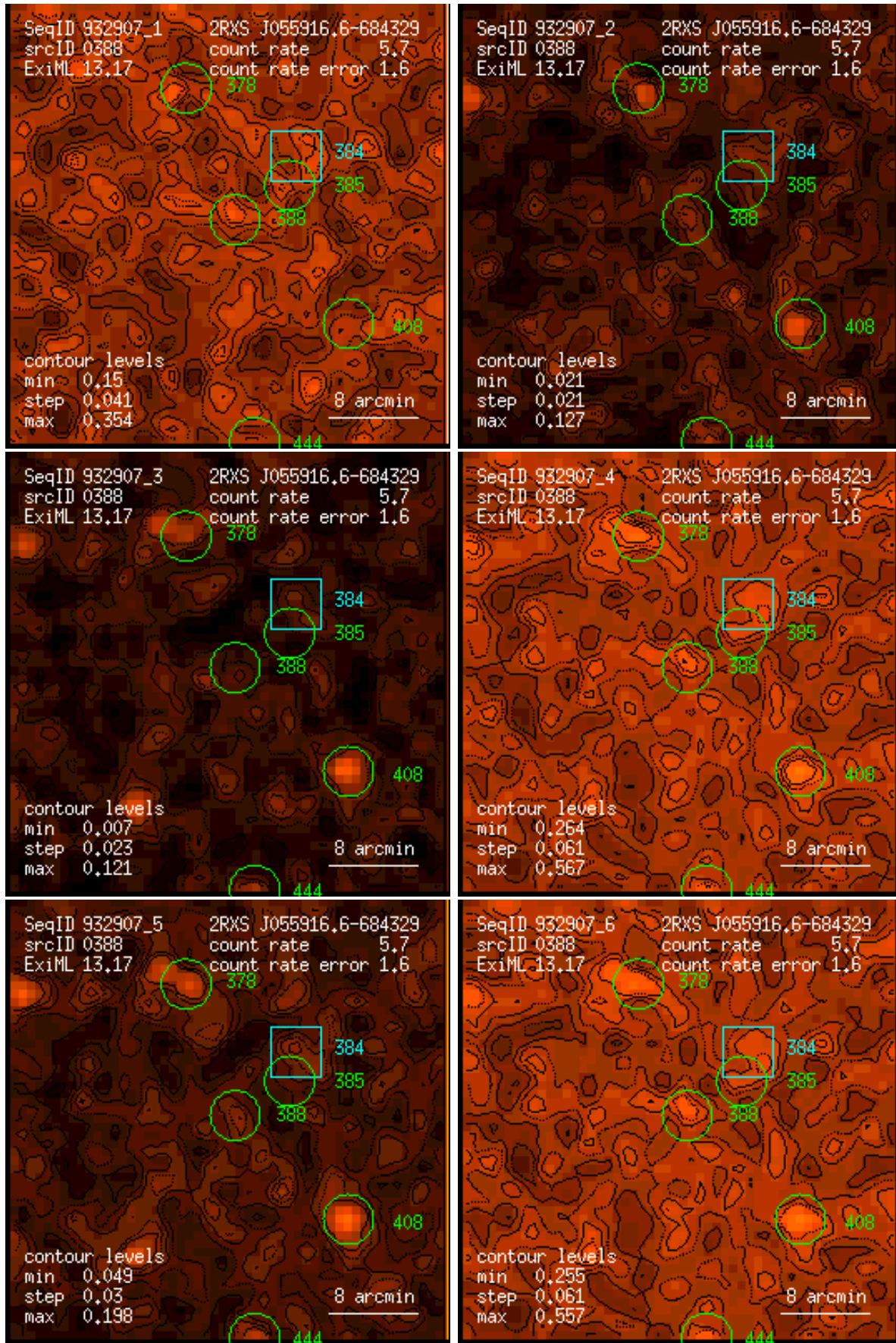
Figure 388: RASS 932907: detection 0388: band rate images, Gaussian filter: (1) PSPC channels 11 – 41, (2) 52 – 90, (3) 91 – 201, (4) 11 – 235, (5) 52 – 201, (6) 11 – 201. Broad band rates in counts/ks. Band rate contour levels in counts/ks/arcmin 2 .
