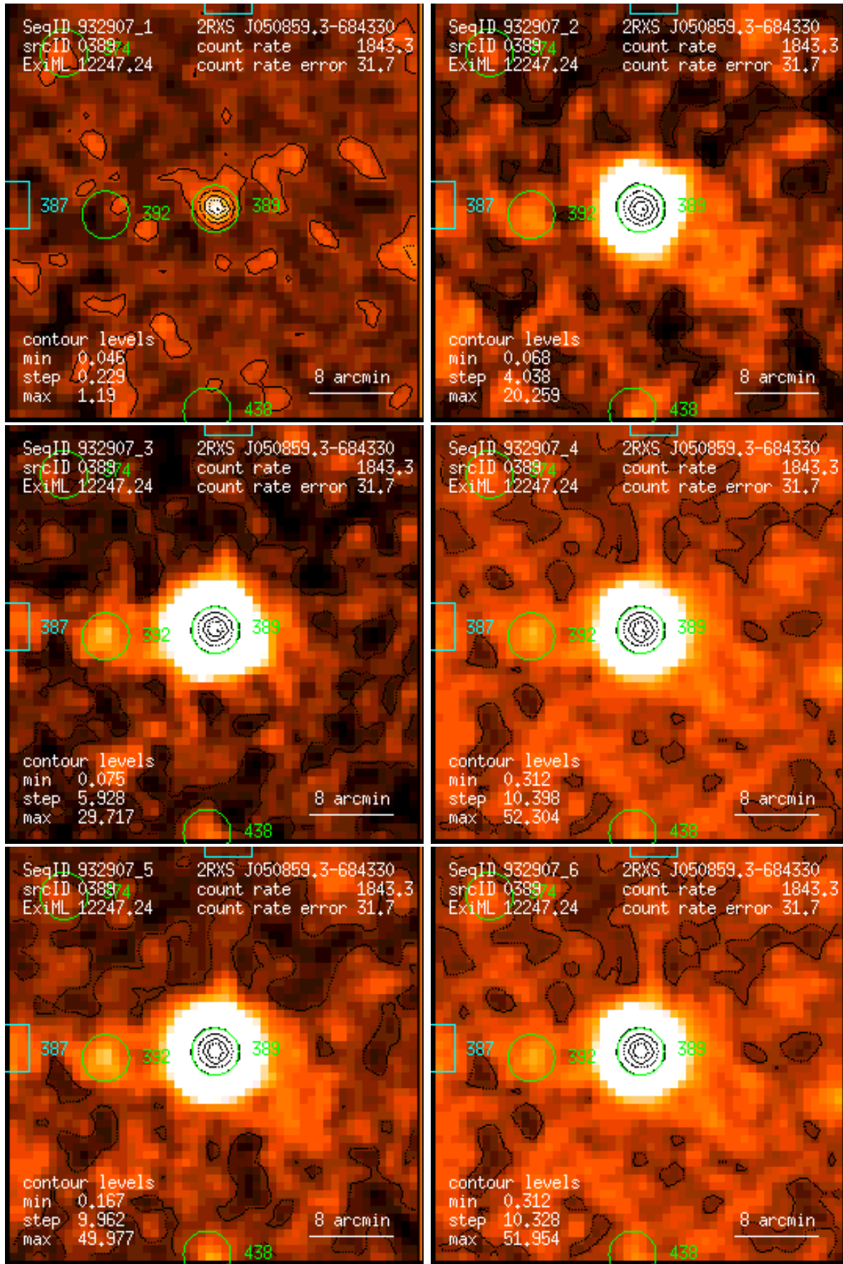
Figure 389: RASS 932907: detection 0389: band rate images, Gaussian filter: (1) PSPC channels 11 – 41, (2) 52 – 90, (3) 91 – 201, (4) 11 – 235, (5) 52 – 201, (6) 11 – 201. Broad band rates in counts/ks. Band rate contour levels in counts/ks/arcmin 2 .
