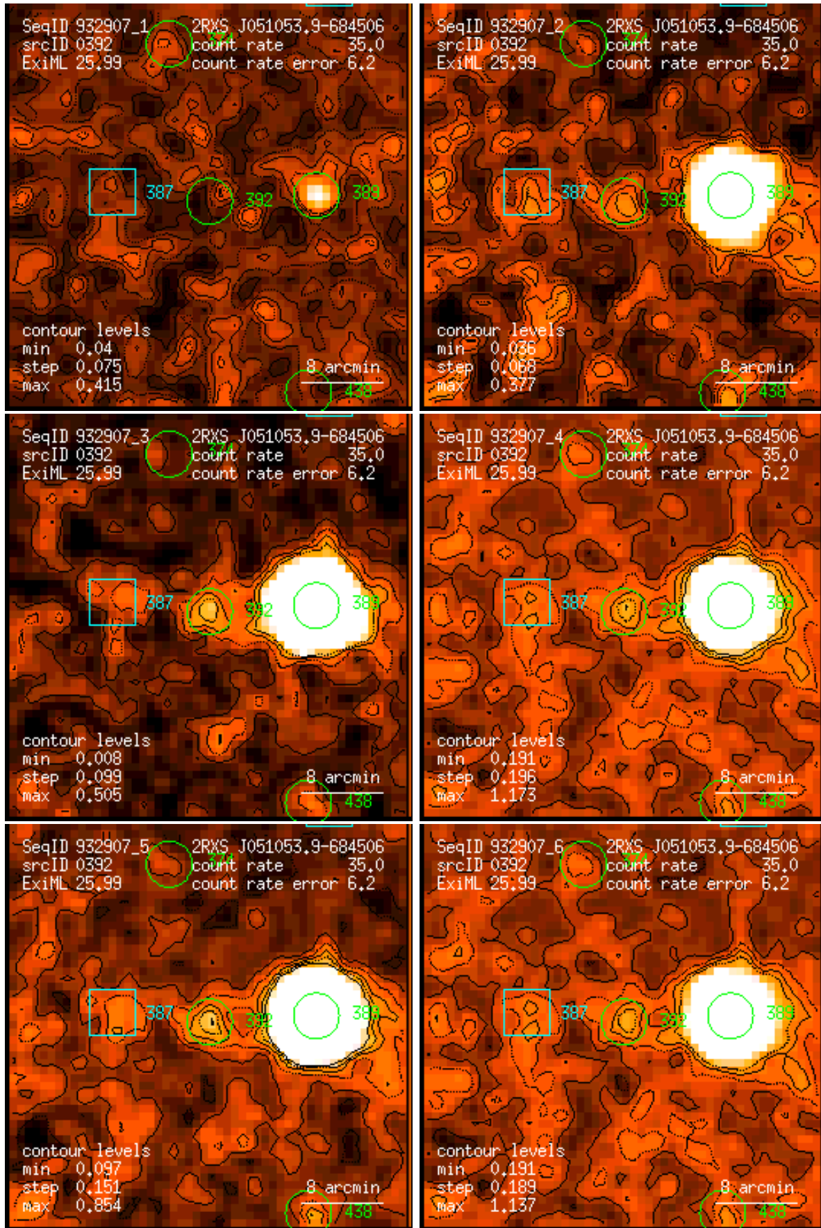
Figure 392: RASS 932907: detection 0392: band rate images, Gaussian filter: (1) PSPC channels 11 – 41, (2) 52 – 90, (3) 91 – 201, (4) 11 – 235, (5) 52 – 201, (6) 11 – 201. Broad band rates in counts/ks. Band rate contour levels in counts/ks/arcmin 2 .
