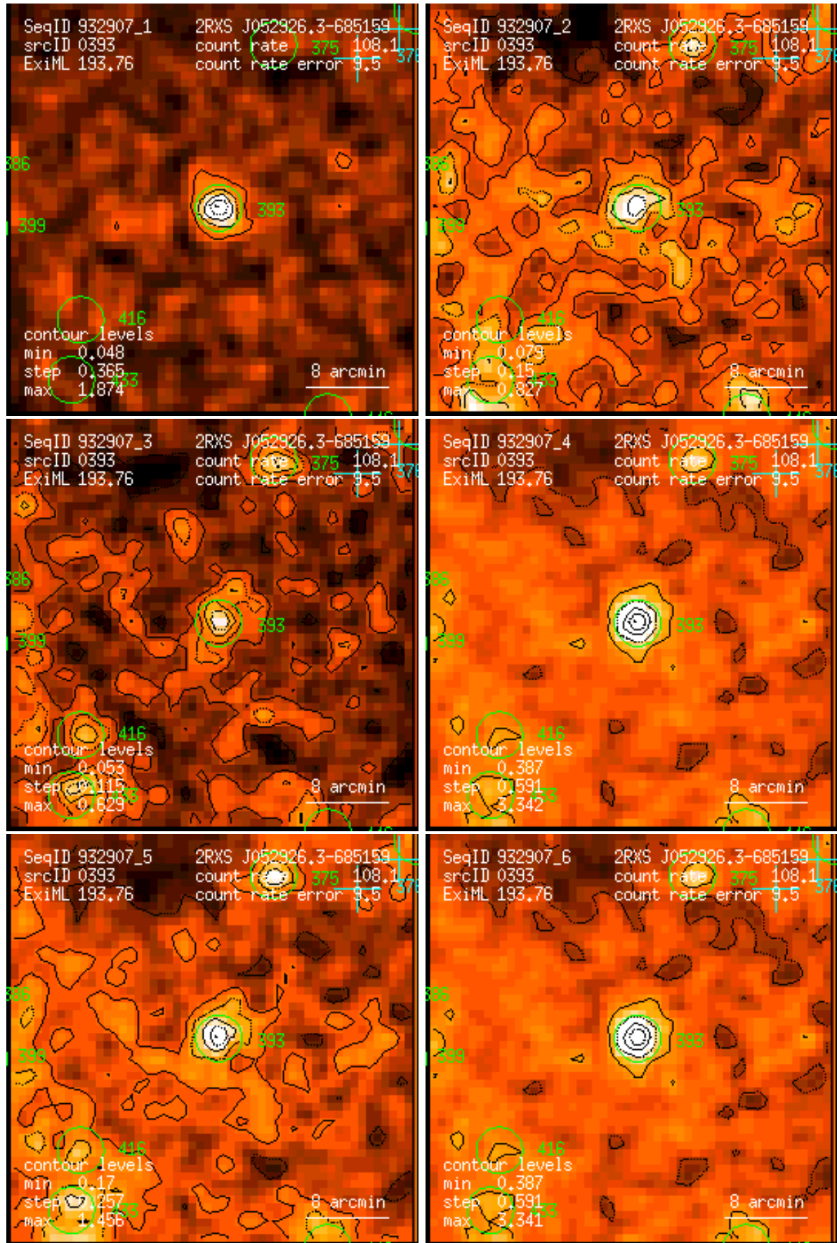
Figure 393: RASS 932907: detection 0393: band rate images, Gaussian filter: (1) PSPC channels 11 – 41, (2) 52 – 90, (3) 91 – 201, (4) 11 – 235, (5) 52 – 201, (6) 11 – 201. Broad band rates in counts/ks. Band rate contour levels in counts/ks/arcmin 2 .
