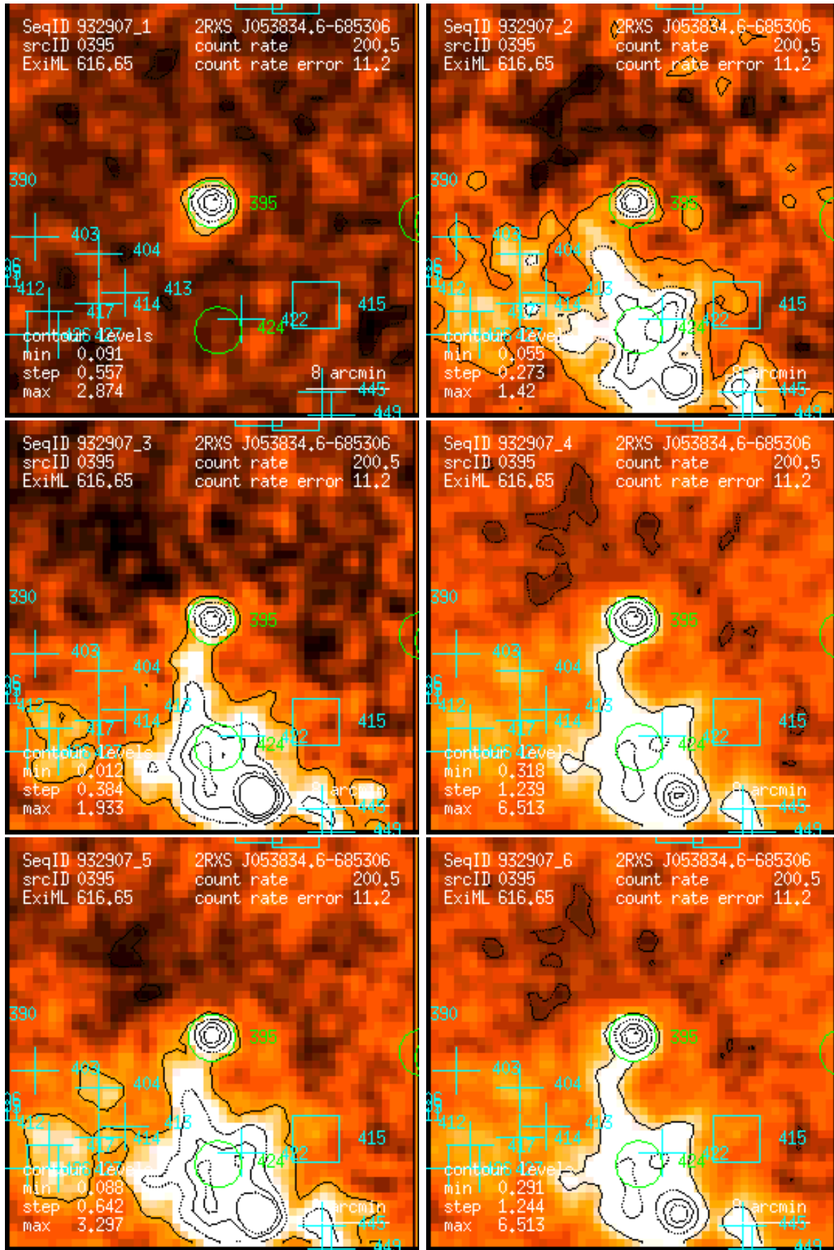
Figure 395: RASS 932907: detection 0395: band rate images, Gaussian filter: (1) PSPC channels 11 – 41, (2) 52 – 90, (3) 91 – 201, (4) 11 – 235, (5) 52 – 201, (6) 11 – 201. Broad band rates in counts/ks. Band rate contour levels in counts/ks/arcmin 2 .
