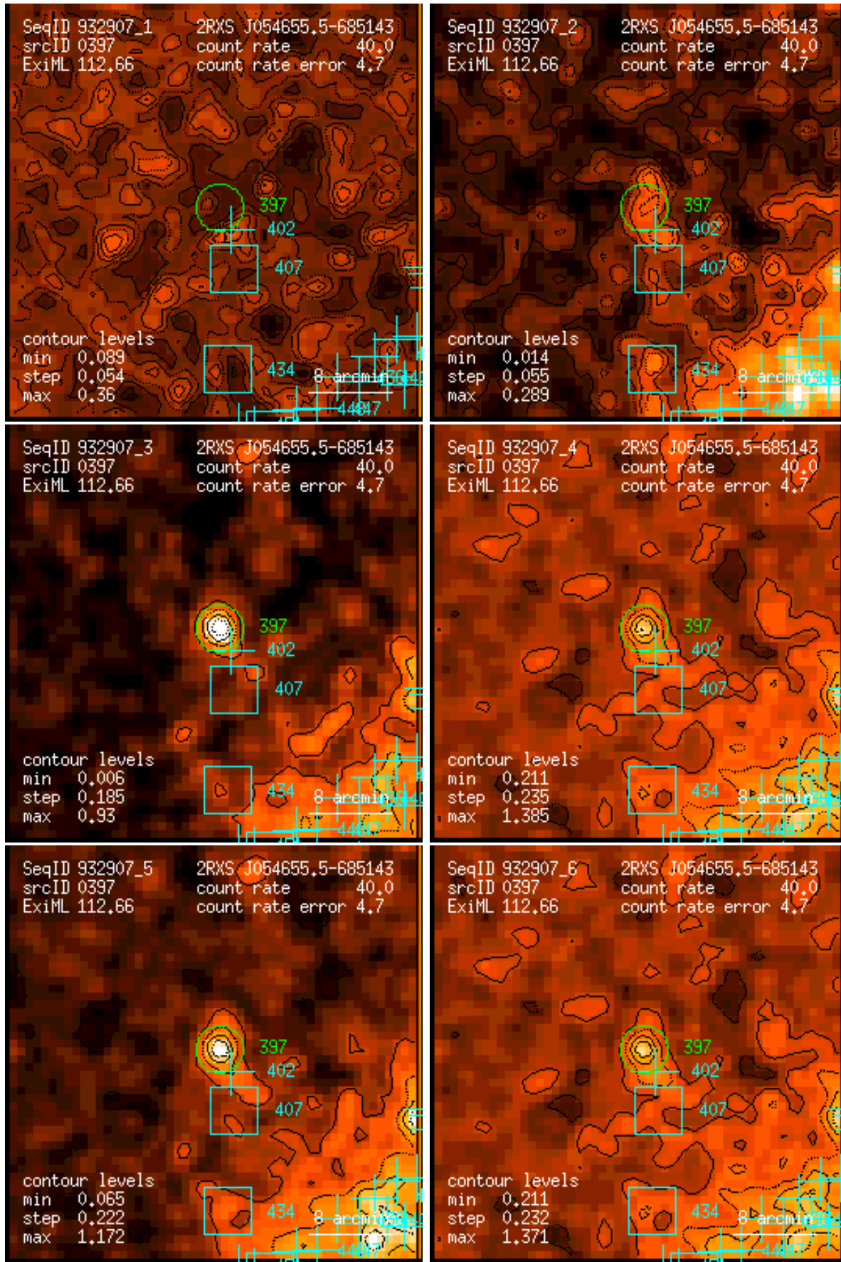
Figure 397: RASS 932907: detection 0397: band rate images, Gaussian filter: (1) PSPC channels 11 – 41, (2) 52 – 90, (3) 91 – 201, (4) 11 – 235, (5) 52 – 201, (6) 11 – 201. Broad band rates in counts/ks. Band rate contour levels in counts/ks/arcmin 2 .
