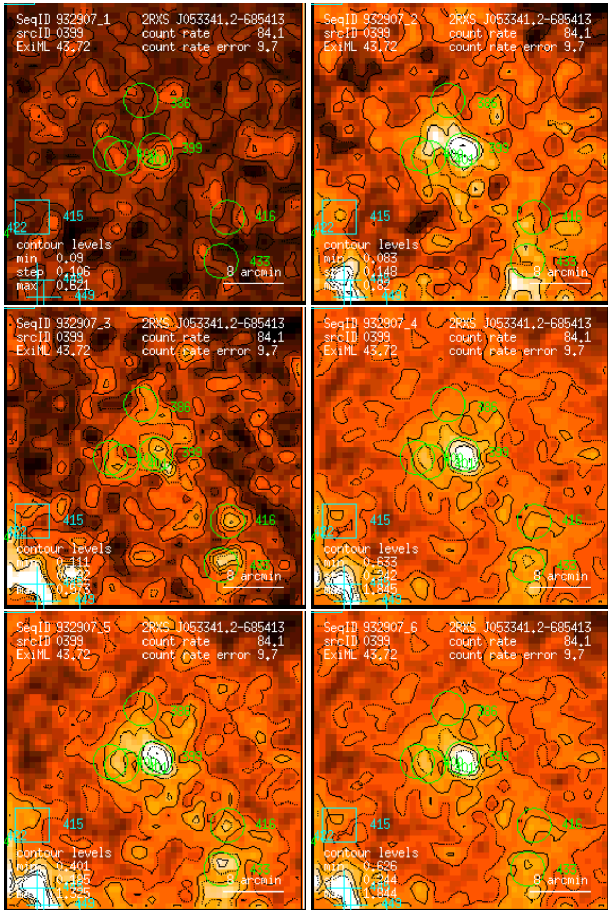
Figure 399: RASS 932907: detection 0399: band rate images, Gaussian filter: (1) PSPC channels 11 – 41, (2) 52 – 90, (3) 91 – 201, (4) 11 – 235, (5) 52 – 201, (6) 11 – 201. Broad band rates in counts/ks. Band rate contour levels in counts/ks/arcmin 2 .
