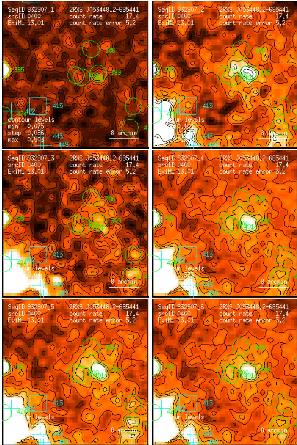
Figure 400: RASS 932907: detection 0400: band rate images, Gaussian filter: (1) PSPC channels 11 – 41, (2) 52 – 90, (3) 91 – 201, (4) 11 – 235, (5) 52 – 201, (6) 11 – 201. Broad band rates in counts/ks. Band rate contour levels in counts/ks/arcmin 2 .
