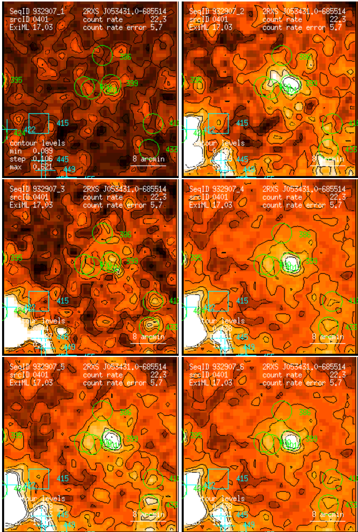
Figure 401: RASS 932907: detection 0401: band rate images, Gaussian filter: (1) PSPC channels 11 – 41, (2) 52 – 90, (3) 91 – 201, (4) 11 – 235, (5) 52 – 201, (6) 11 – 201. Broad band rates in counts/ks. Band rate contour levels in counts/ks/arcmin 2 .
