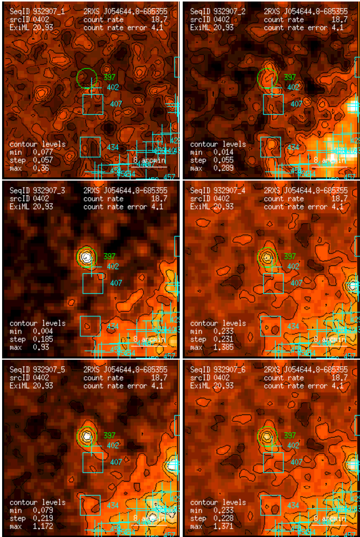
Figure 402: RASS 932907: detection 0402: band rate images, Gaussian filter: (1) PSPC channels 11 – 41, (2) 52 – 90, (3) 91 – 201, (4) 11 – 235, (5) 52 – 201, (6) 11 – 201. Broad band rates in counts/ks. Band rate contour levels in counts/ks/arcmin 2 .
