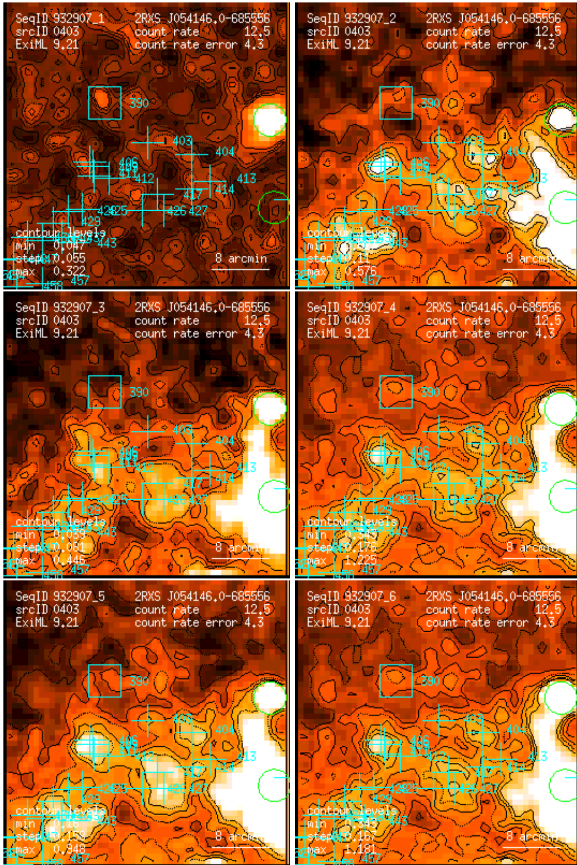
Figure 403: RASS 932907: detection 0403: band rate images, Gaussian filter: (1) PSPC channels 11 – 41, (2) 52 – 90, (3) 91 – 201, (4) 11 – 235, (5) 52 – 201, (6) 11 – 201. Broad band rates in counts/ks. Band rate contour levels in counts/ks/arcmin 2 .
