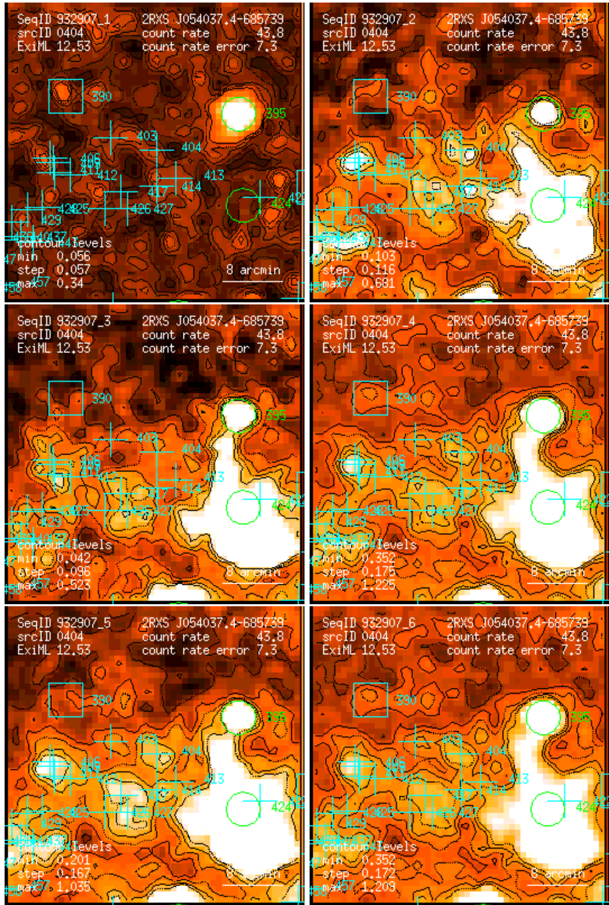
Figure 404: RASS 932907: detection 0404: band rate images, Gaussian filter: (1) PSPC channels 11 – 41, (2) 52 – 90, (3) 91 – 201, (4) 11 – 235, (5) 52 – 201, (6) 11 – 201. Broad band rates in counts/ks. Band rate contour levels in counts/ks/arcmin 2 .
