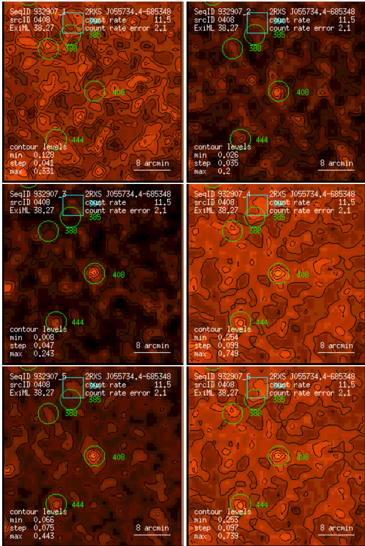
Figure 408: RASS 932907: detection 0408: band rate images, Gaussian filter: (1) PSPC channels 11 – 41, (2) 52 – 90, (3) 91 – 201, (4) 11 – 235, (5) 52 – 201, (6) 11 – 201. Broad band rates in counts/ks. Band rate contour levels in counts/ks/arcmin 2 .
