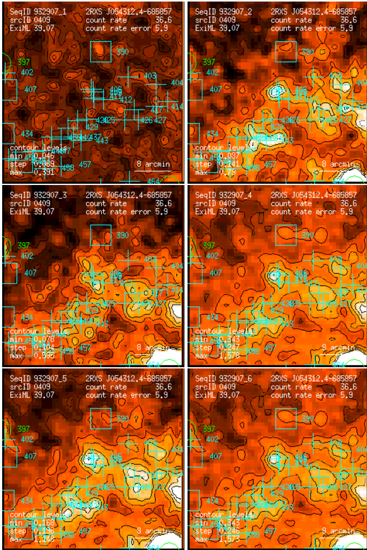
Figure 409: RASS 932907: detection 0409: band rate images, Gaussian filter: (1) PSPC channels 11 – 41, (2) 52 – 90, (3) 91 – 201, (4) 11 – 235, (5) 52 – 201, (6) 11 – 201. Broad band rates in counts/ks. Band rate contour levels in counts/ks/arcmin 2 .
