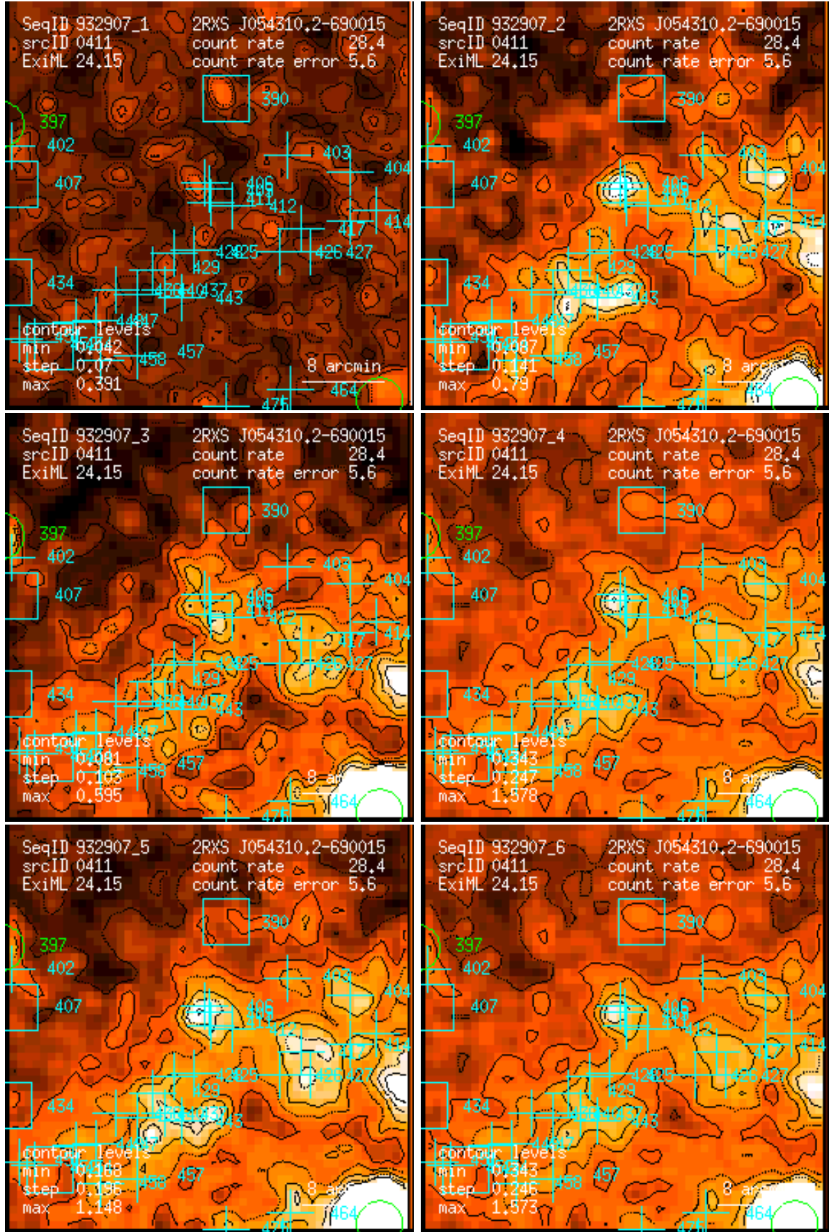
Figure 411: RASS 932907: detection 0411: band rate images, Gaussian filter: (1) PSPC channels 11 – 41, (2) 52 – 90, (3) 91 – 201, (4) 11 – 235, (5) 52 – 201, (6) 11 – 201. Broad band rates in counts/ks. Band rate contour levels in counts/ks/arcmin 2 .
