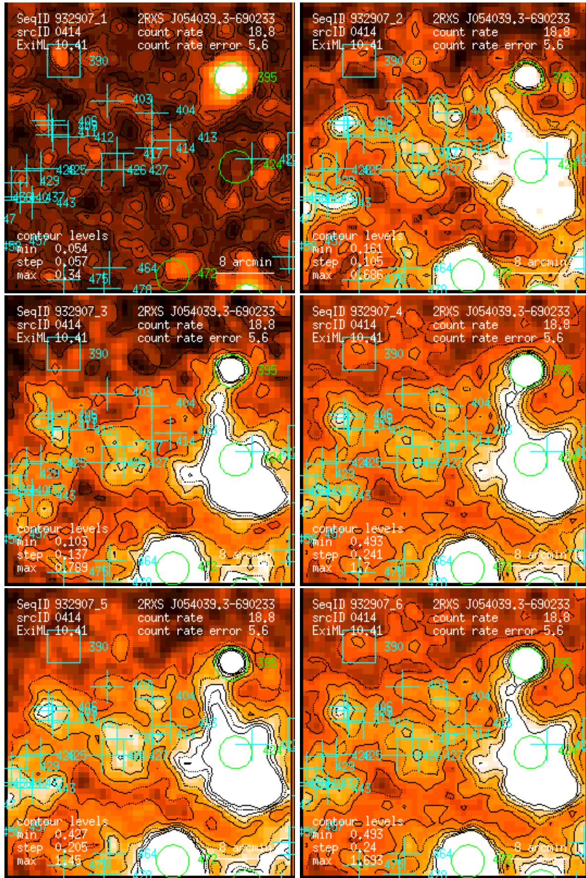
Figure 414: RASS 932907: detection 0414: band rate images, Gaussian filter: (1) PSPC channels 11 – 41, (2) 52 – 90, (3) 91 – 201, (4) 11 – 235, (5) 52 – 201, (6) 11 – 201. Broad band rates in counts/ks. Band rate contour levels in counts/ks/arcmin 2 .
