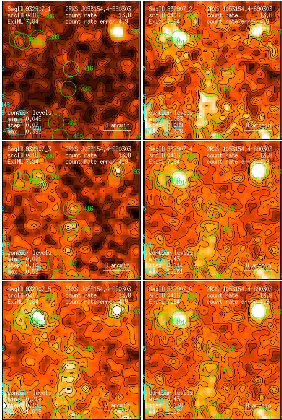
Figure 416: RASS 932907: detection 0416: band rate images, Gaussian filter: (1) PSPC channels 11 – 41, (2) 52 – 90, (3) 91 – 201, (4) 11 – 235, (5) 52 – 201, (6) 11 – 201. Broad band rates in counts/ks. Band rate contour levels in counts/ks/arcmin 2 .
