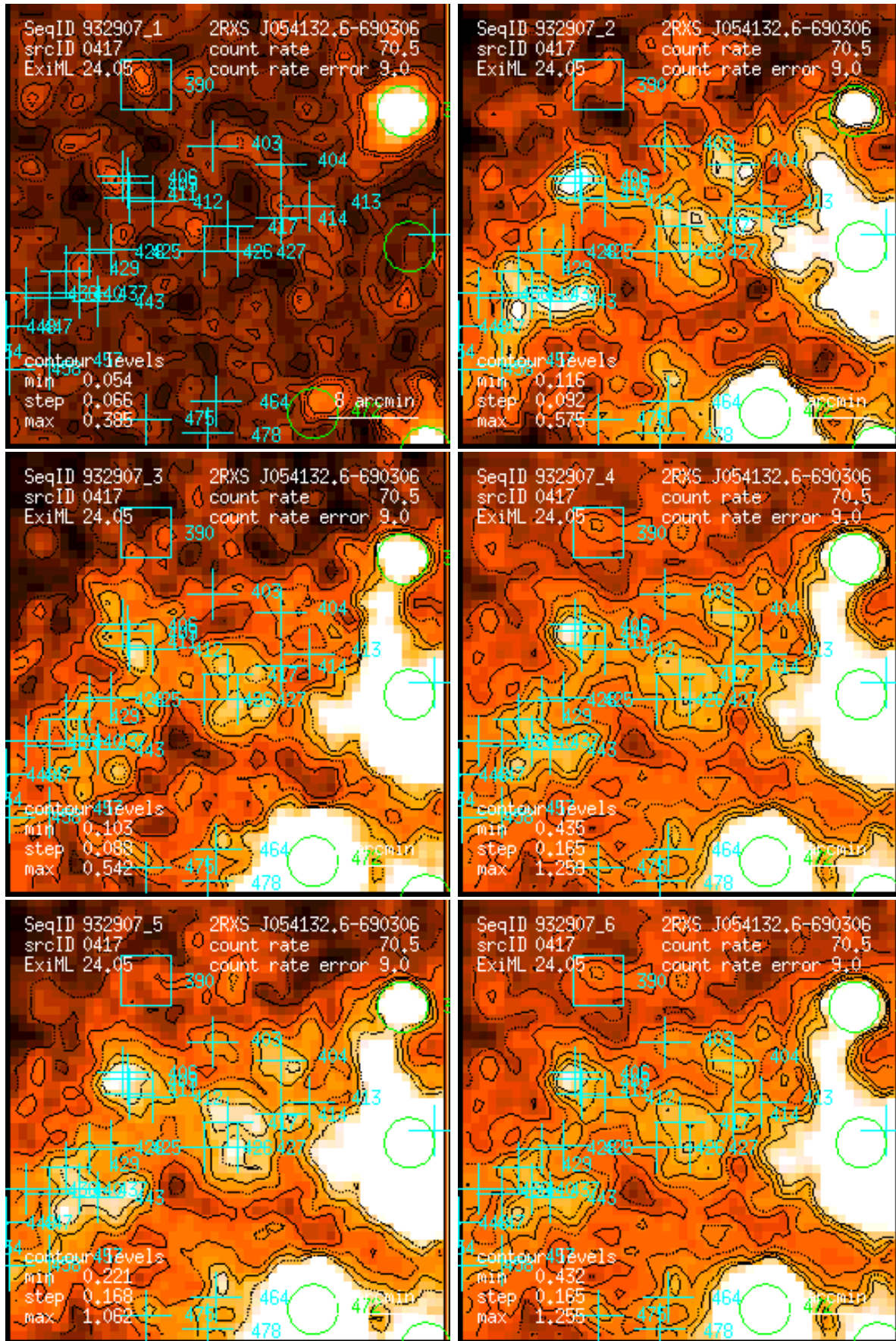
Figure 417: RASS 932907: detection 0417: band rate images, Gaussian filter: (1) PSPC channels 11 – 41, (2) 52 – 90, (3) 91 – 201, (4) 11 – 235, (5) 52 – 201, (6) 11 – 201. Broad band rates in counts/ks. Band rate contour levels in counts/ks/arcmin 2 .
