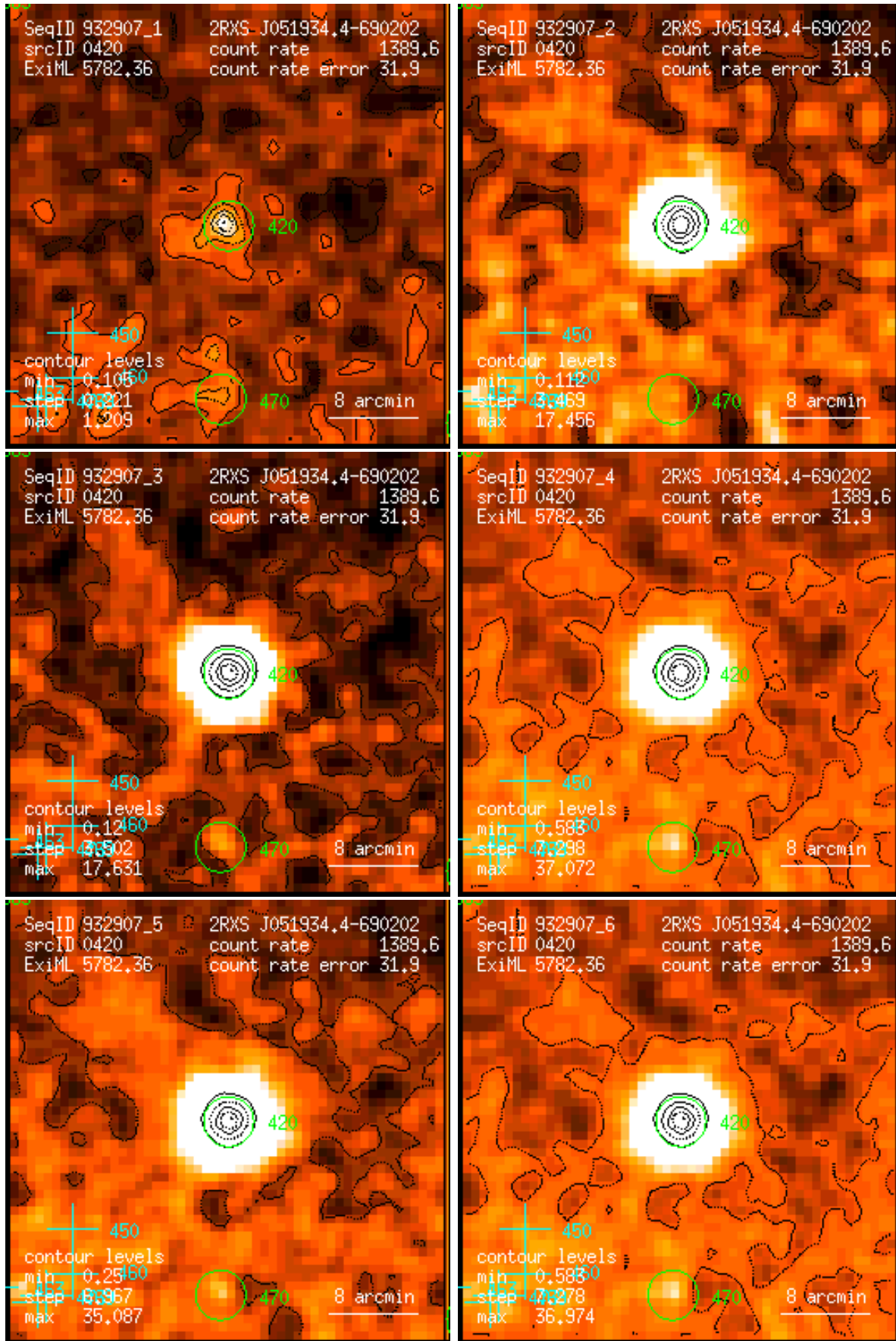
Figure 420: RASS 932907: detection 0420: band rate images, Gaussian filter: (1) PSPC channels 11 – 41, (2) 52 – 90, (3) 91 – 201, (4) 11 – 235, (5) 52 – 201, (6) 11 – 201. Broad band rates in counts/ks. Band rate contour levels in counts/ks/arcmin 2 .
