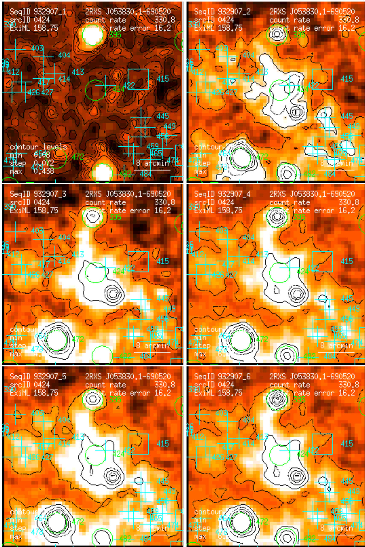
Figure 424: RASS 932907: detection 0424: band rate images, Gaussian filter: (1) PSPC channels 11 – 41, (2) 52 – 90, (3) 91 – 201, (4) 11 – 235, (5) 52 – 201, (6) 11 – 201. Broad band rates in counts/ks. Band rate contour levels in counts/ks/arcmin 2 .
