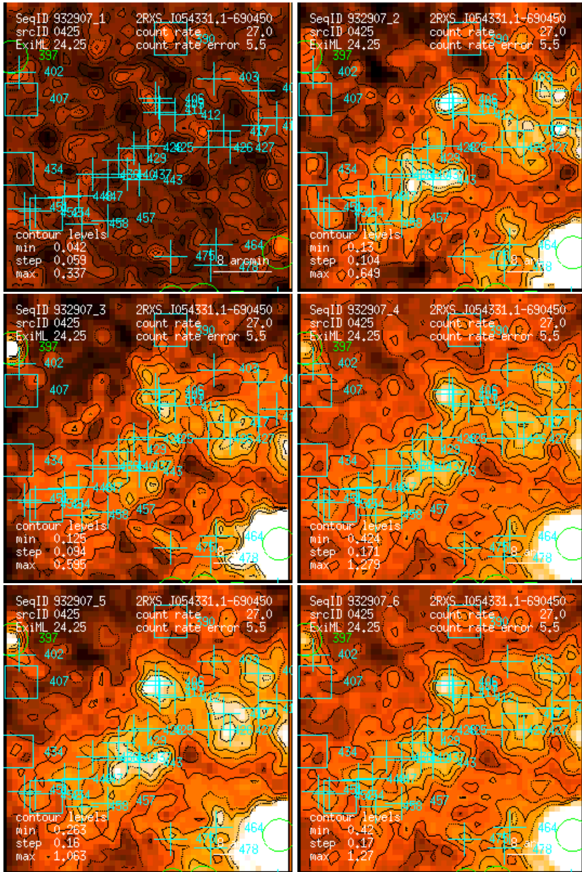
Figure 425: RASS 932907: detection 0425: band rate images, Gaussian filter: (1) PSPC channels 11 – 41, (2) 52 – 90, (3) 91 – 201, (4) 11 – 235, (5) 52 – 201, (6) 11 – 201. Broad band rates in counts/ks. Band rate contour levels in counts/ks/arcmin 2 .
