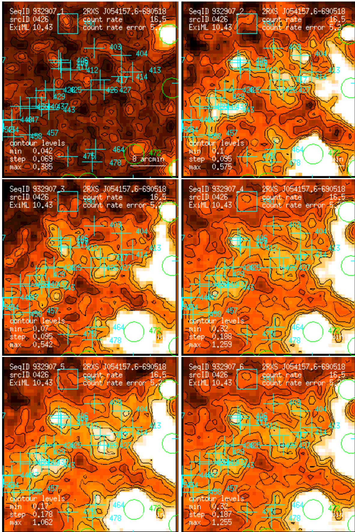
Figure 426: RASS 932907: detection 0426: band rate images, Gaussian filter: (1) PSPC channels 11 – 41, (2) 52 – 90, (3) 91 – 201, (4) 11 – 235, (5) 52 – 201, (6) 11 – 201. Broad band rates in counts/ks. Band rate contour levels in counts/ks/arcmin 2 .
