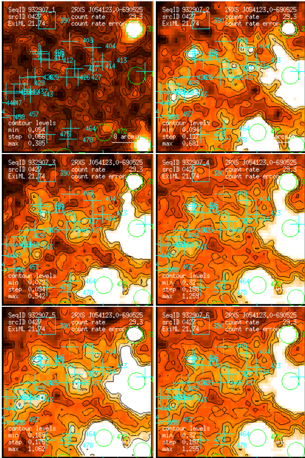
Figure 427: RASS 932907: detection 0427: band rate images, Gaussian filter: (1) PSPC channels 11 – 41, (2) 52 – 90, (3) 91 – 201, (4) 11 – 235, (5) 52 – 201, (6) 11 – 201. Broad band rates in counts/ks. Band rate contour levels in counts/ks/arcmin 2 .
