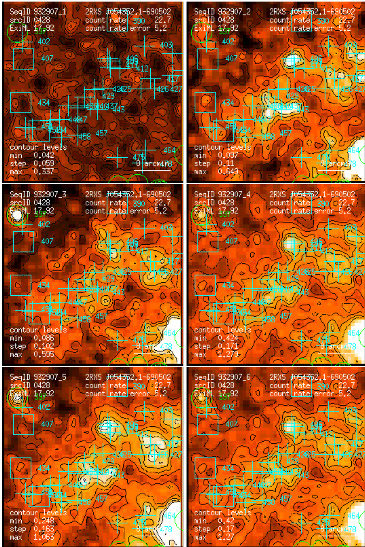
Figure 428: RASS 932907: detection 0428: band rate images, Gaussian filter: (1) PSPC channels 11 – 41, (2) 52 – 90, (3) 91 – 201, (4) 11 – 235, (5) 52 – 201, (6) 11 – 201. Broad band rates in counts/ks. Band rate contour levels in counts/ks/arcmin 2 .
