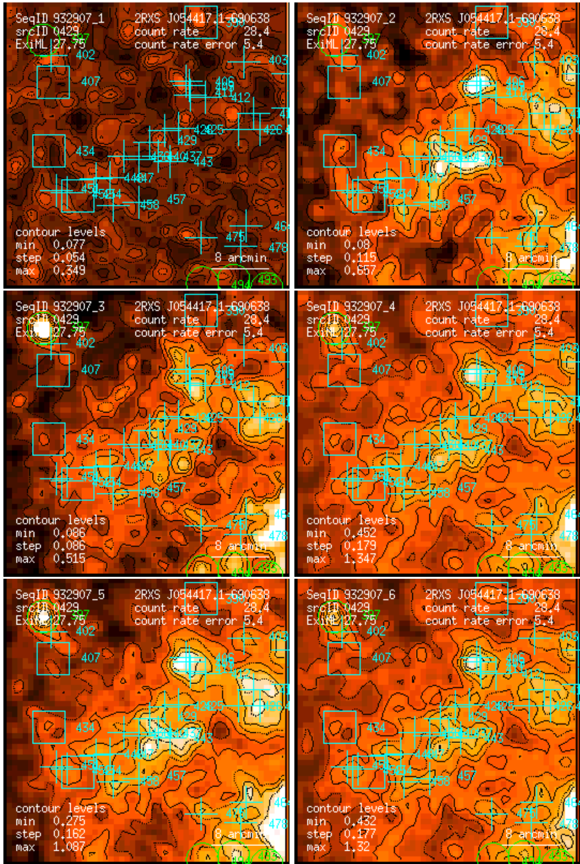
Figure 429: RASS 932907: detection 0429: band rate images, Gaussian filter: (1) PSPC channels 11 – 41, (2) 52 – 90, (3) 91 – 201, (4) 11 – 235, (5) 52 – 201, (6) 11 – 201. Broad band rates in counts/ks. Band rate contour levels in counts/ks/arcmin 2 .
