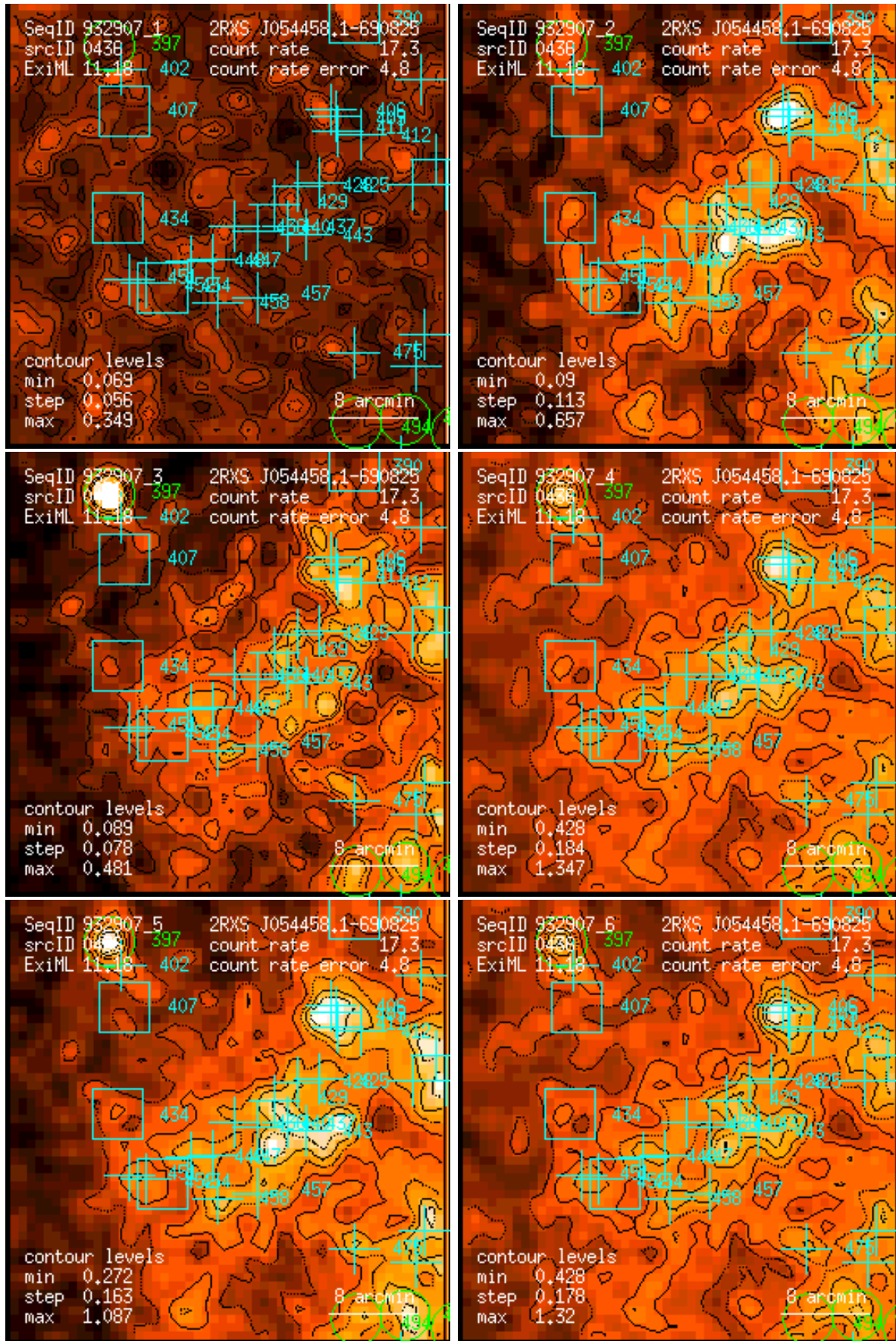
Figure 436: RASS 932907: detection 0436: band rate images, Gaussian filter: (1) PSPC channels 11 – 41, (2) 52 – 90, (3) 91 – 201, (4) 11 – 235, (5) 52 – 201, (6) 11 – 201. Broad band rates in counts/ks. Band rate contour levels in counts/ks/arcmin 2 .
