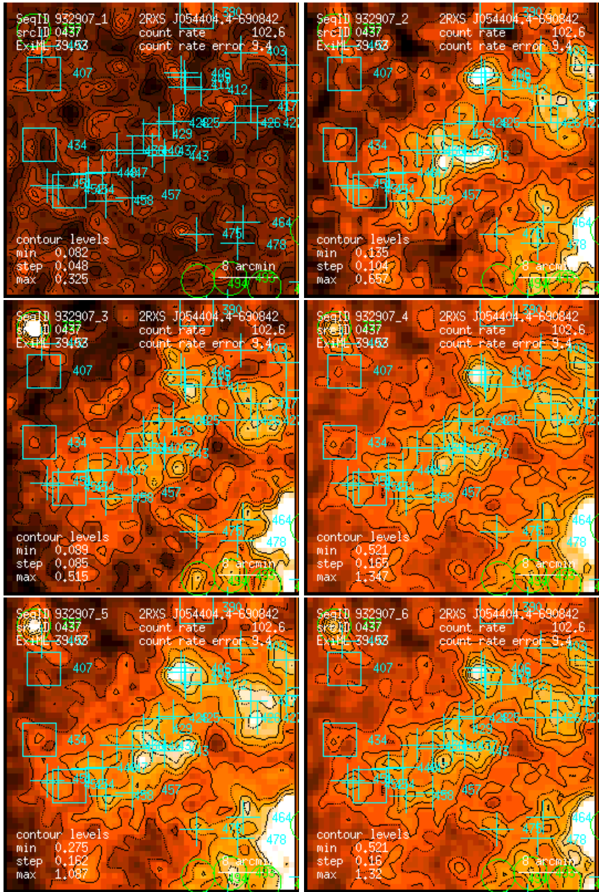
Figure 437: RASS 932907: detection 0437: band rate images, Gaussian filter: (1) PSPC channels 11 – 41, (2) 52 – 90, (3) 91 – 201, (4) 11 – 235, (5) 52 – 201, (6) 11 – 201. Broad band rates in counts/ks. Band rate contour levels in counts/ks/arcmin 2 .
