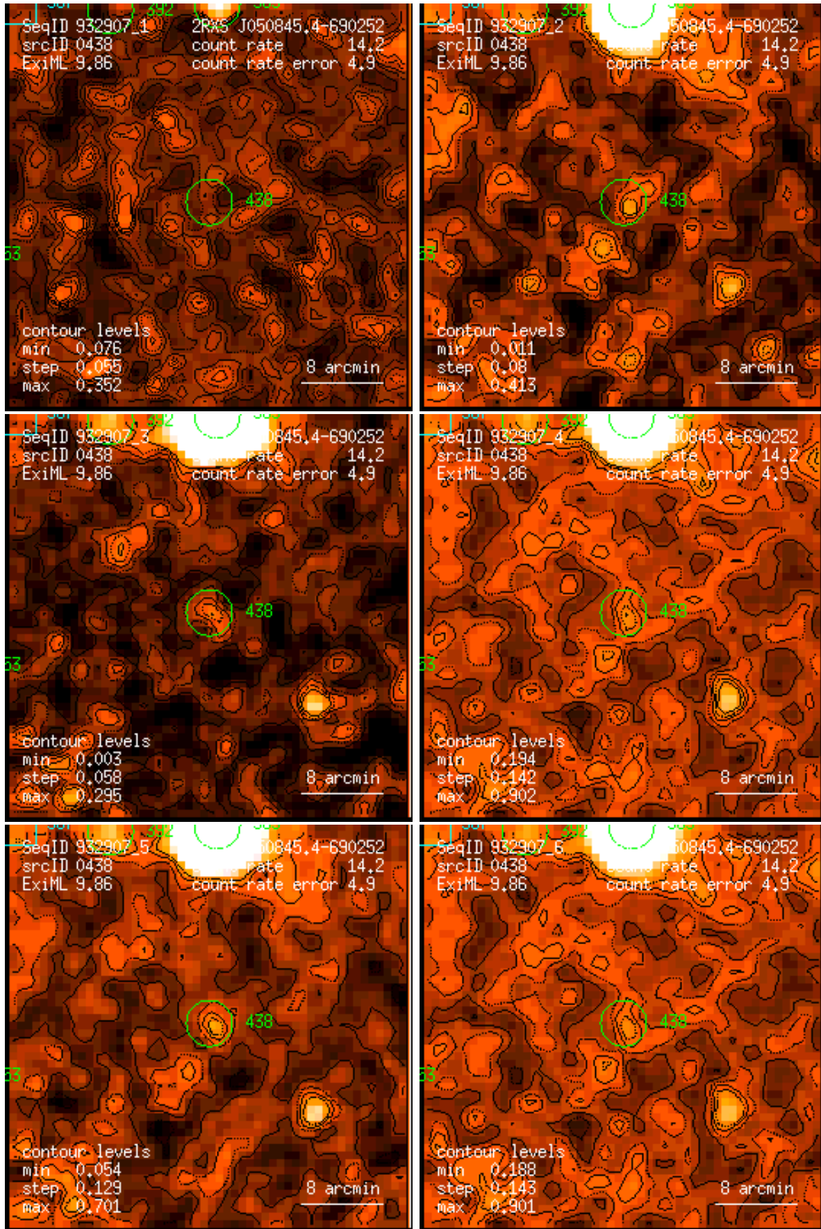
Figure 438: RASS 932907: detection 0438: band rate images, Gaussian filter: (1) PSPC channels 11 – 41, (2) 52 – 90, (3) 91 – 201, (4) 11 – 235, (5) 52 – 201, (6) 11 – 201. Broad band rates in counts/ks. Band rate contour levels in counts/ks/arcmin 2 .
