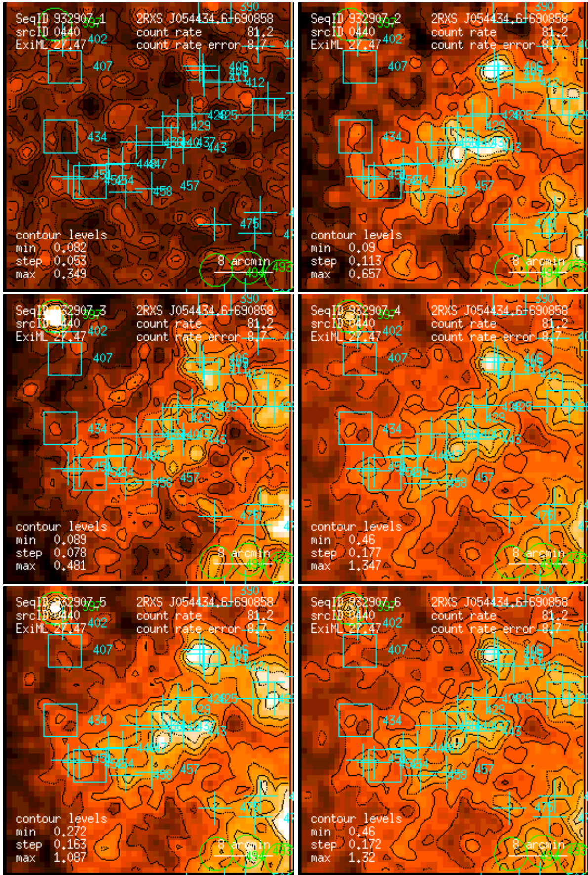
Figure 440: RASS 932907: detection 0440: band rate images, Gaussian filter: (1) PSPC channels 11 – 41, (2) 52 – 90, (3) 91 – 201, (4) 11 – 235, (5) 52 – 201, (6) 11 – 201. Broad band rates in counts/ks. Band rate contour levels in counts/ks/arcmin 2 .
