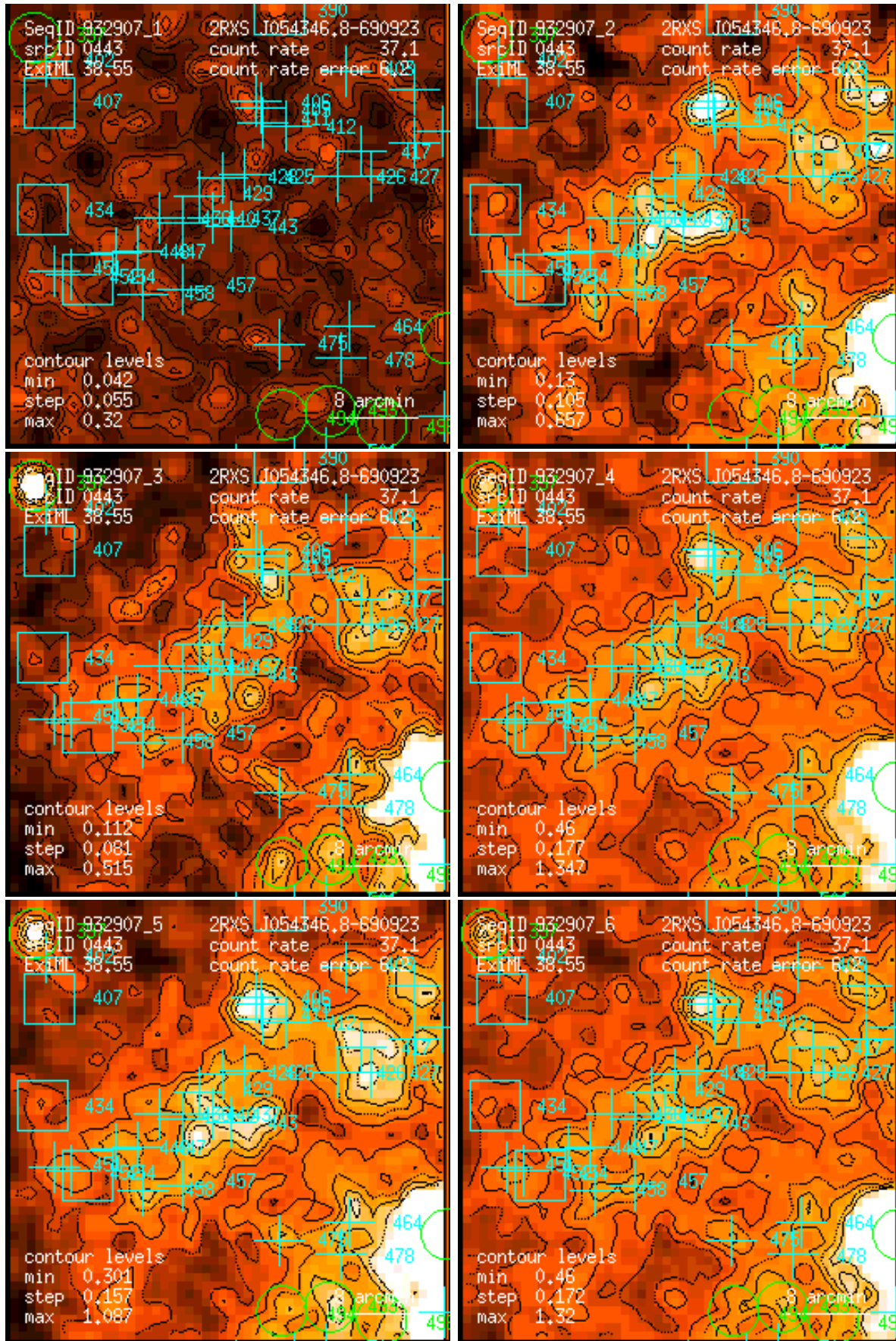
Figure 443: RASS 932907: detection 0443: band rate images, Gaussian filter: (1) PSPC channels 11 – 41, (2) 52 – 90, (3) 91 – 201, (4) 11 – 235, (5) 52 – 201, (6) 11 – 201. Broad band rates in counts/ks. Band rate contour levels in counts/ks/arcmin 2 .
