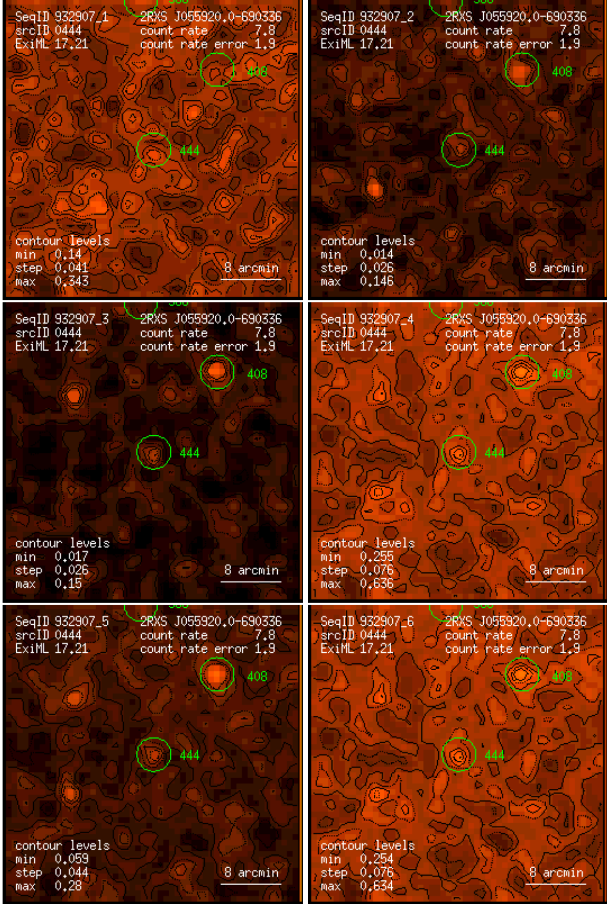
Figure 444: RASS 932907: detection 0444: band rate images, Gaussian filter: (1) PSPC channels 11 – 41, (2) 52 – 90, (3) 91 – 201, (4) 11 – 235, (5) 52 – 201, (6) 11 – 201. Broad band rates in counts/ks. Band rate contour levels in counts/ks/arcmin 2 .
