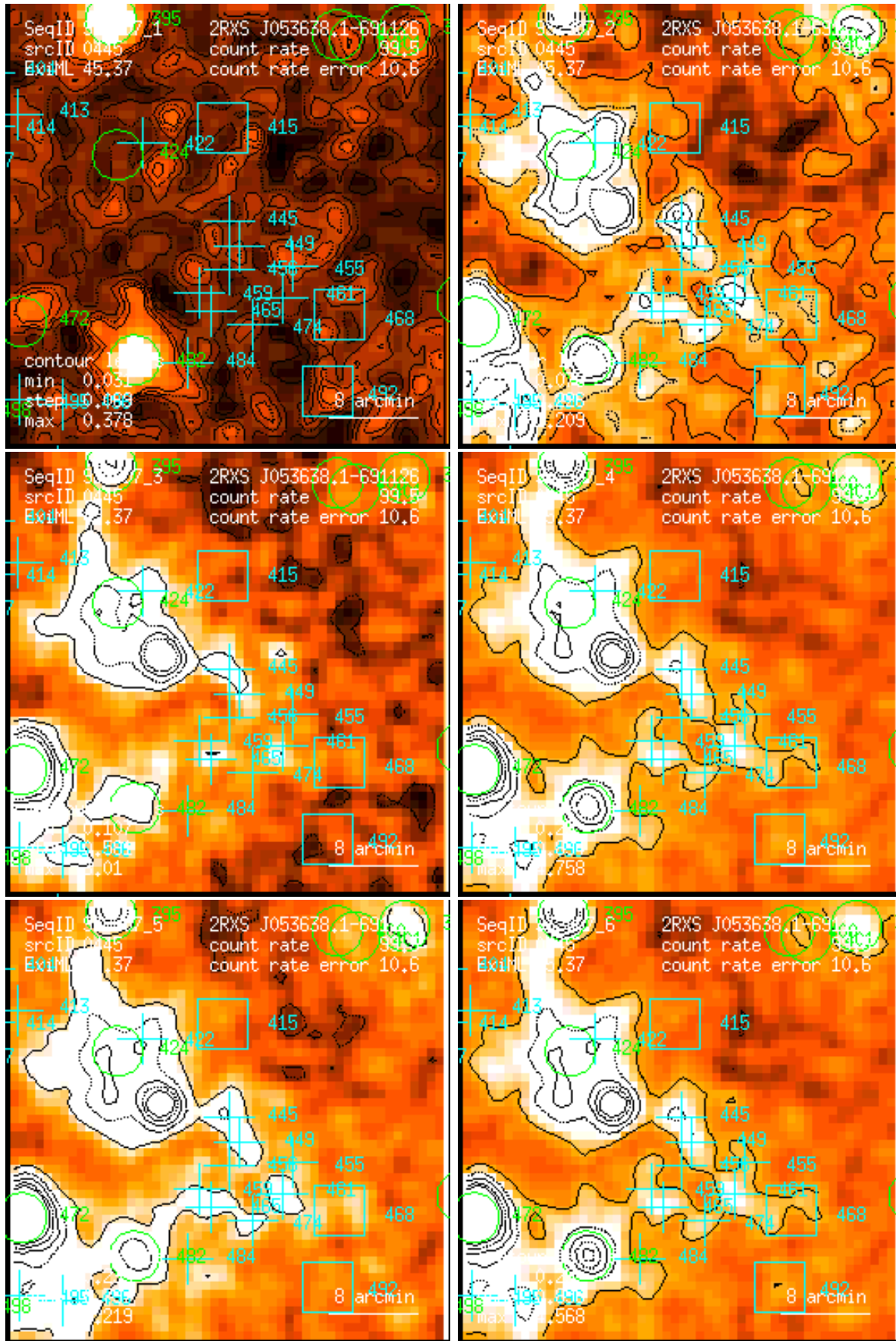
Figure 445: RASS 932907: detection 0445: band rate images, Gaussian filter: (1) PSPC channels 11 – 41, (2) 52 – 90, (3) 91 – 201, (4) 11 – 235, (5) 52 – 201, (6) 11 – 201. Broad band rates in counts/ks. Band rate contour levels in counts/ks/arcmin 2 .
