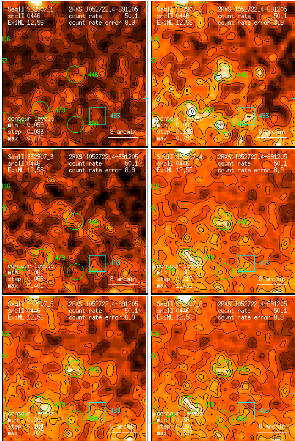
Figure 446: RASS 932907: detection 0446: band rate images, Gaussian filter: (1) PSPC channels 11 – 41, (2) 52 – 90, (3) 91 – 201, (4) 11 – 235, (5) 52 – 201, (6) 11 – 201. Broad band rates in counts/ks. Band rate contour levels in counts/ks/arcmin 2 .
