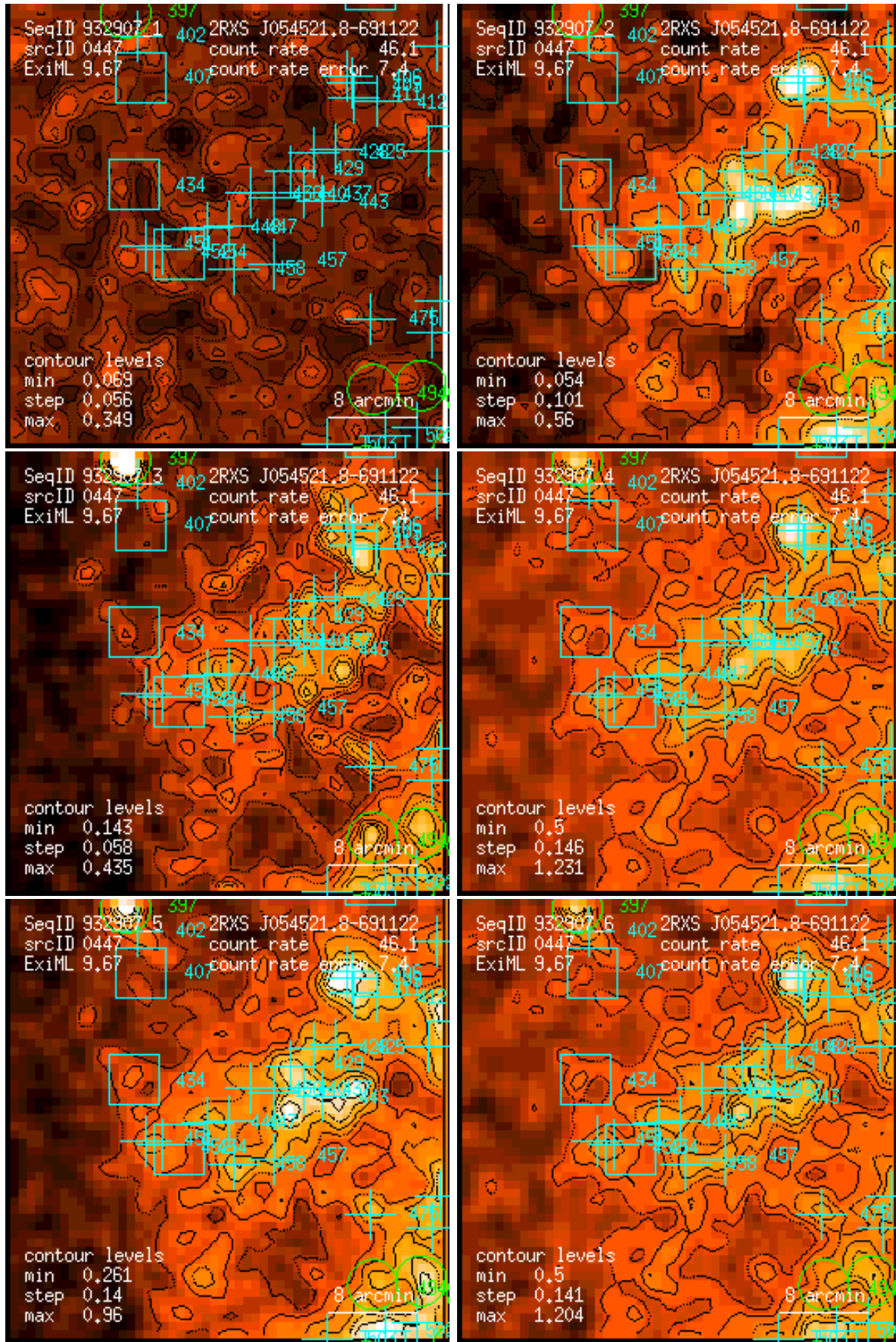
Figure 447: RASS 932907: detection 0447: band rate images, Gaussian filter: (1) PSPC channels 11 – 41, (2) 52 – 90, (3) 91 – 201, (4) 11 – 235, (5) 52 – 201, (6) 11 – 201. Broad band rates in counts/ks. Band rate contour levels in counts/ks/arcmin 2 .
