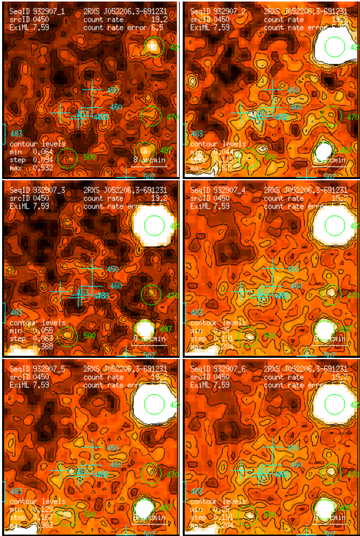
Figure 450: RASS 932907: detection 0450: band rate images, Gaussian filter: (1) PSPC channels 11 – 41, (2) 52 – 90, (3) 91 – 201, (4) 11 – 235, (5) 52 – 201, (6) 11 – 201. Broad band rates in counts/ks. Band rate contour levels in counts/ks/arcmin 2 .
