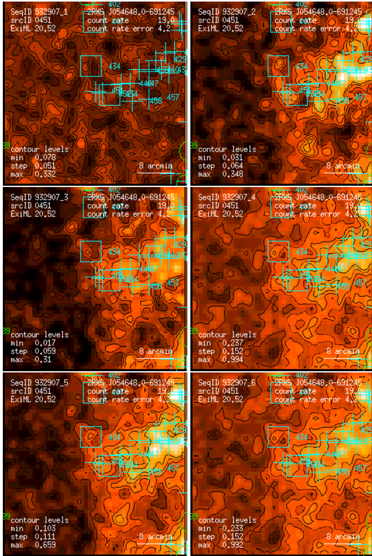
Figure 451: RASS 932907: detection 0451: band rate images, Gaussian filter: (1) PSPC channels 11 – 41, (2) 52 – 90, (3) 91 – 201, (4) 11 – 235, (5) 52 – 201, (6) 11 – 201. Broad band rates in counts/ks. Band rate contour levels in counts/ks/arcmin 2 .
