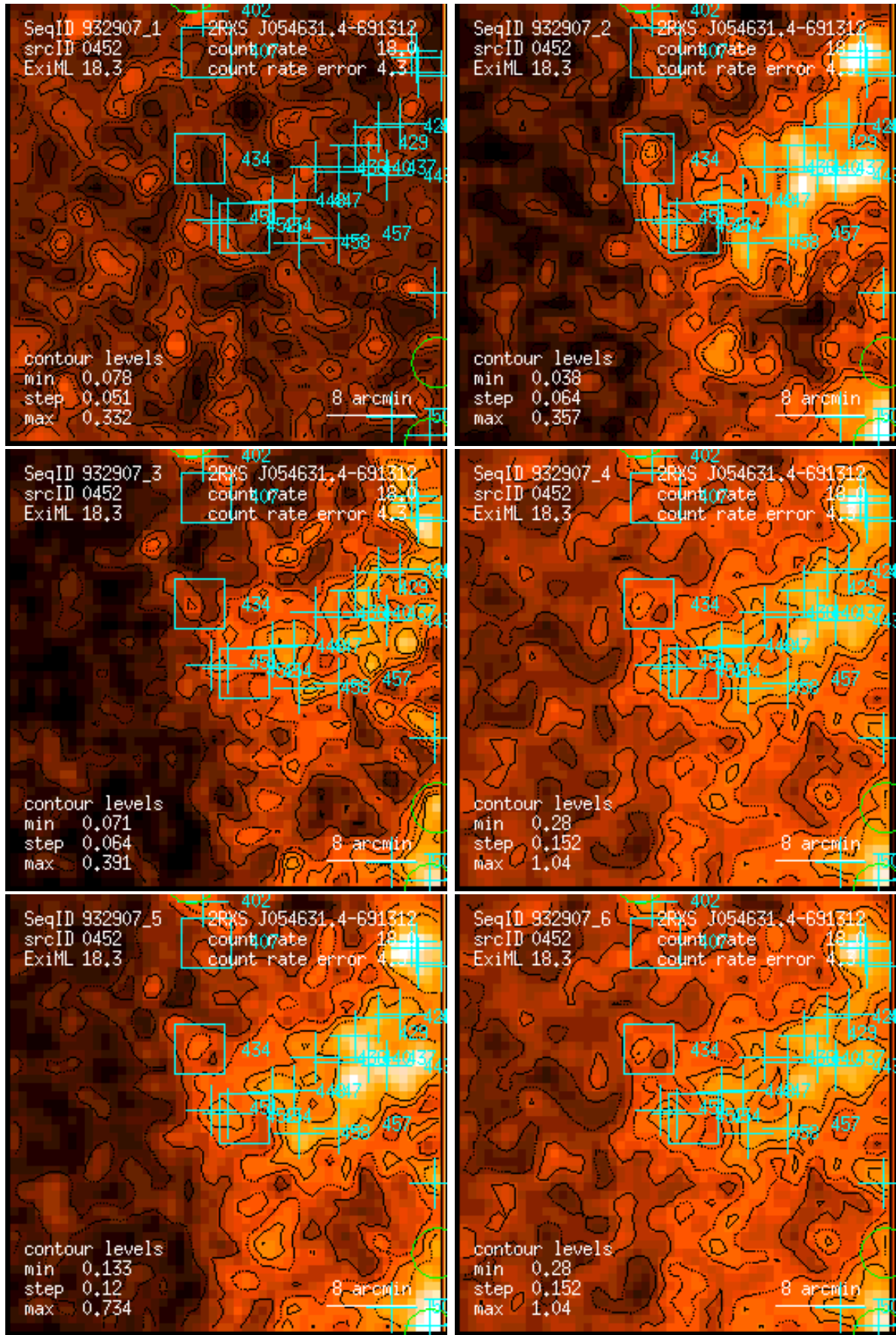
Figure 452: RASS 932907: detection 0452: band rate images, Gaussian filter: (1) PSPC channels 11 – 41, (2) 52 – 90, (3) 91 – 201, (4) 11 – 235, (5) 52 – 201, (6) 11 – 201. Broad band rates in counts/ks. Band rate contour levels in counts/ks/arcmin 2 .
