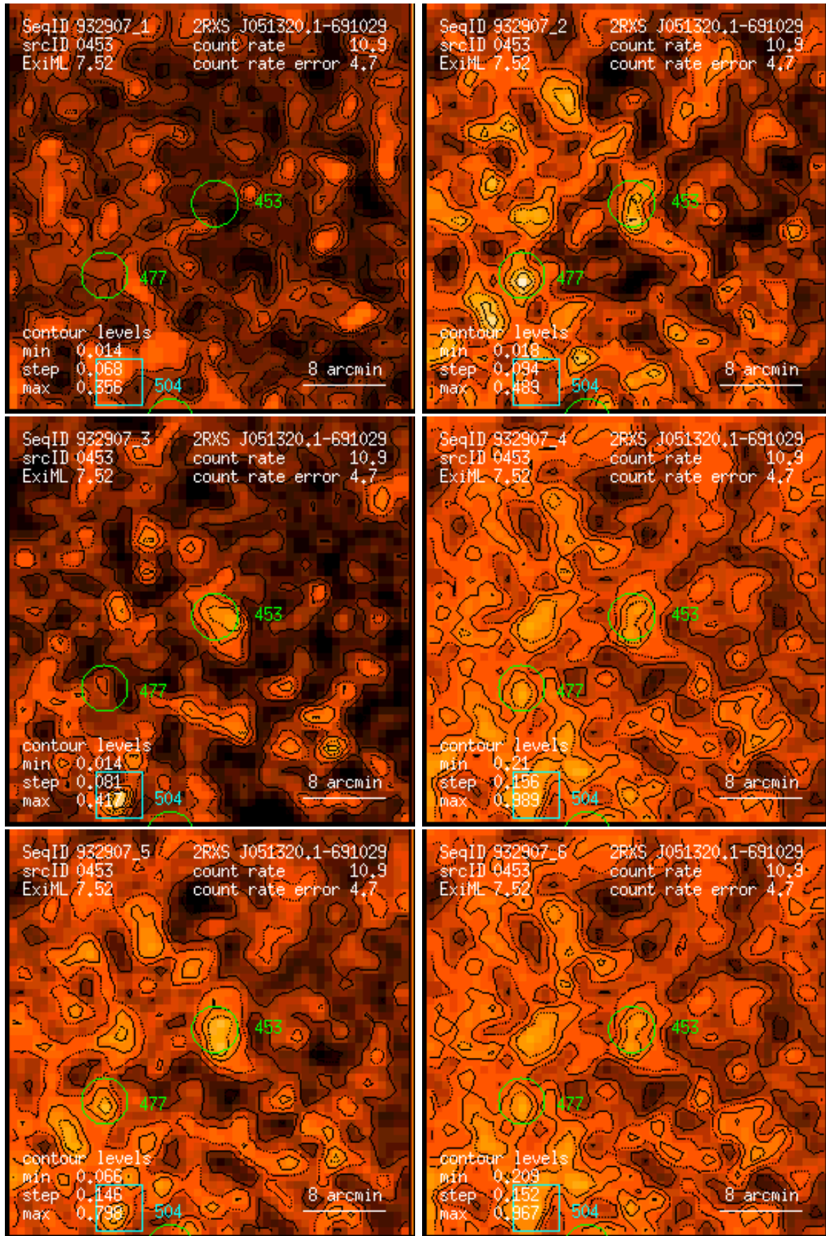
Figure 453: RASS 932907: detection 0453: band rate images, Gaussian filter: (1) PSPC channels 11 – 41, (2) 52 – 90, (3) 91 – 201, (4) 11 – 235, (5) 52 – 201, (6) 11 – 201. Broad band rates in counts/ks. Band rate contour levels in counts/ks/arcmin 2 .
