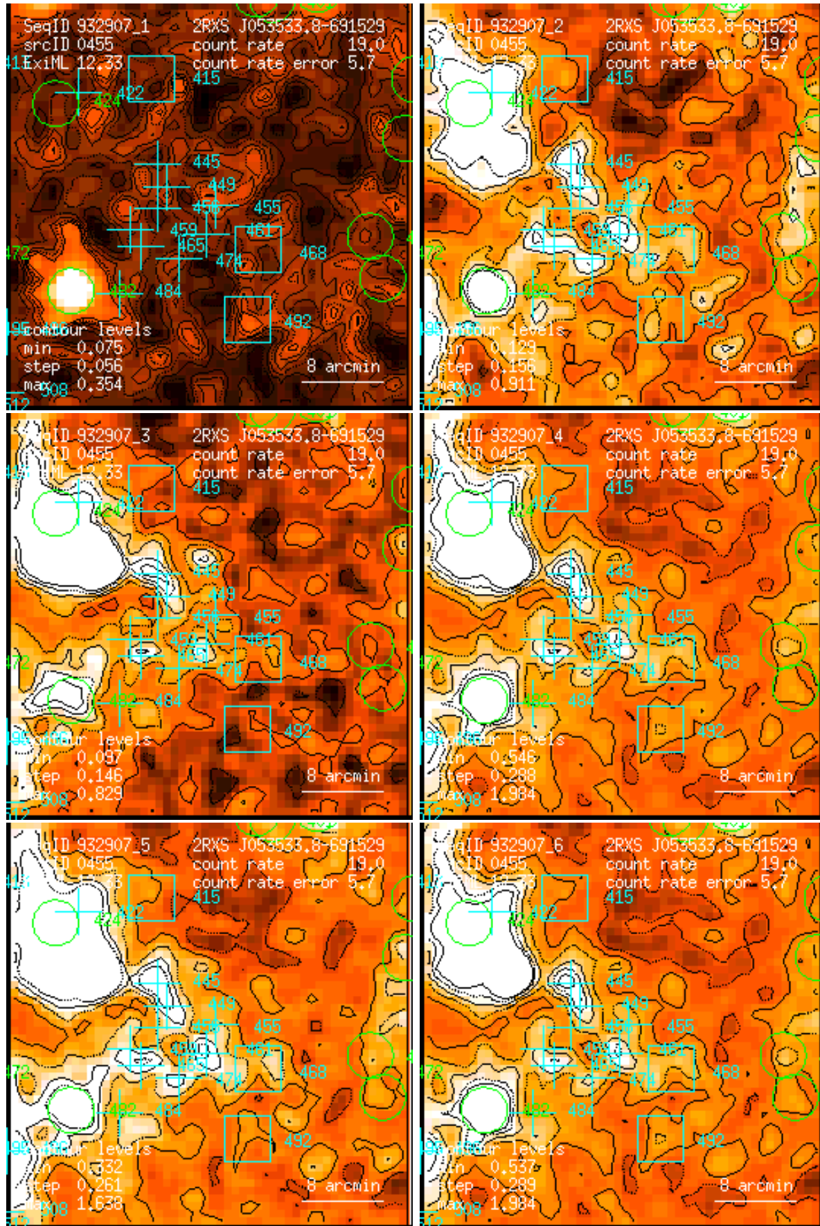
Figure 455: RASS 932907: detection 0455: band rate images, Gaussian filter: (1) PSPC channels 11 – 41, (2) 52 – 90, (3) 91 – 201, (4) 11 – 235, (5) 52 – 201, (6) 11 – 201. Broad band rates in counts/ks. Band rate contour levels in counts/ks/arcmin 2 .
